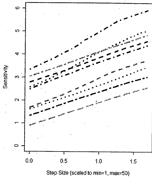
(a) Sensitivities for the three 3D component layout problems
