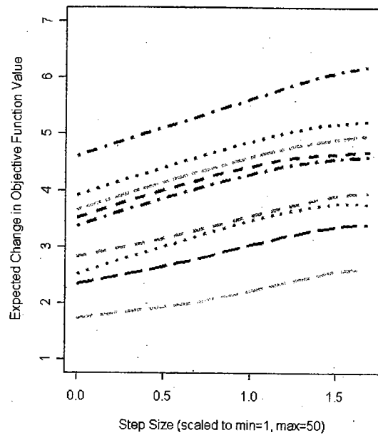
(b) Expected change in objective function value for packing into a spherical container
