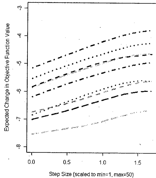
(d) Expected change in objective function value for packing minimizing moment about centroid
