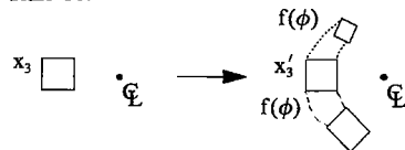
Rule 80:
