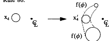
Rule 86:
