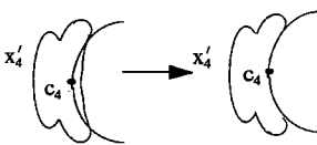
Figure 7 (continued)
