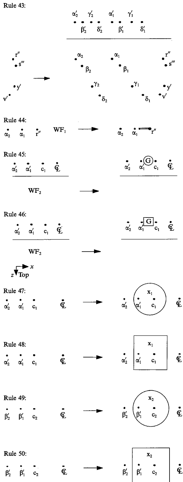
Figure 7. Completion rules.
