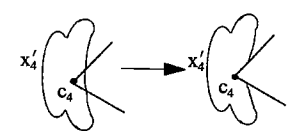
Rule 100:
