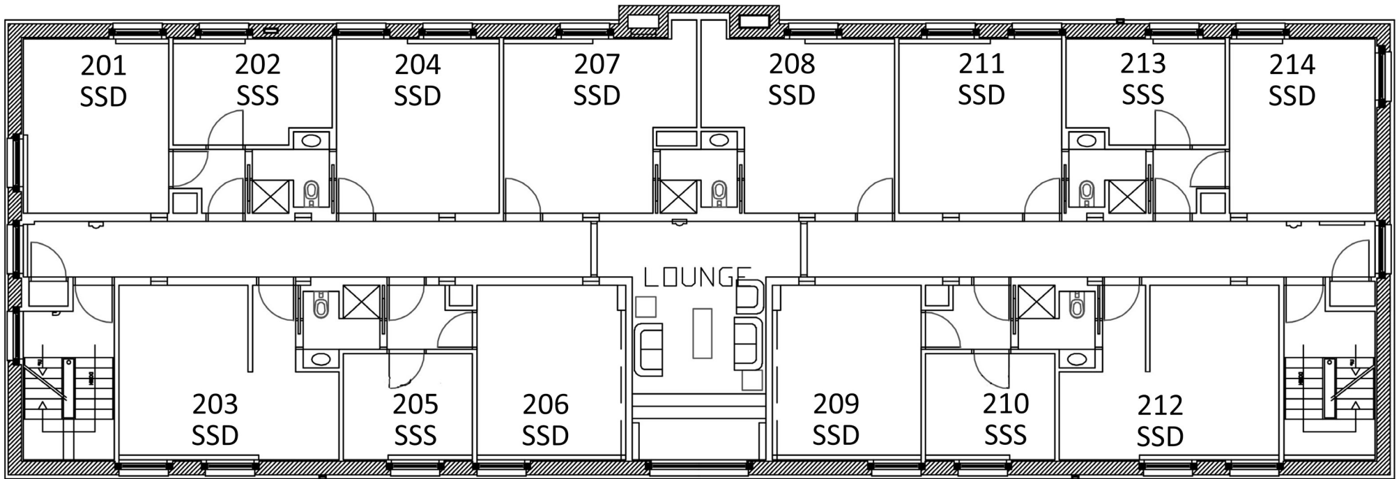
MCGILL SECOND FLOOR LOUNGE 1'0" = 1/8"
