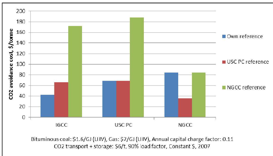
Figure E2. Cost of CO 2 avoidance based on various reference plant technologies
