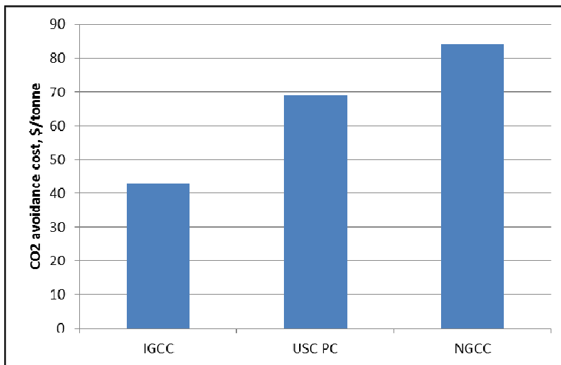
Figure E1. Costs of CO 2 avoidance based on a reference plant of the given technology
