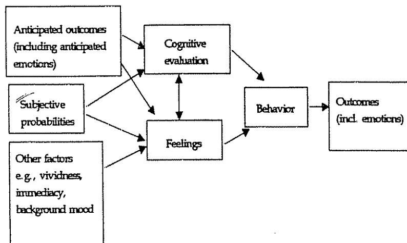
Figure 3 Risk-as-feelings perspective
