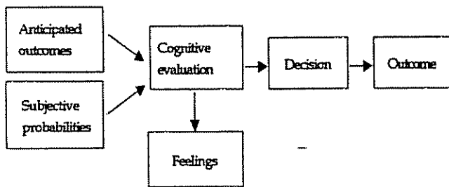
Figure 1. Consequentialist perspective.
