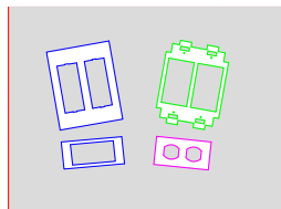
LEFT: V4049 DEVICE MOUNTING BRACKET AND TRIM PLATE. ALSO, 5507D RECTANGULAR AND 5507D DUPLEX FACE PLATE INSERTS.
