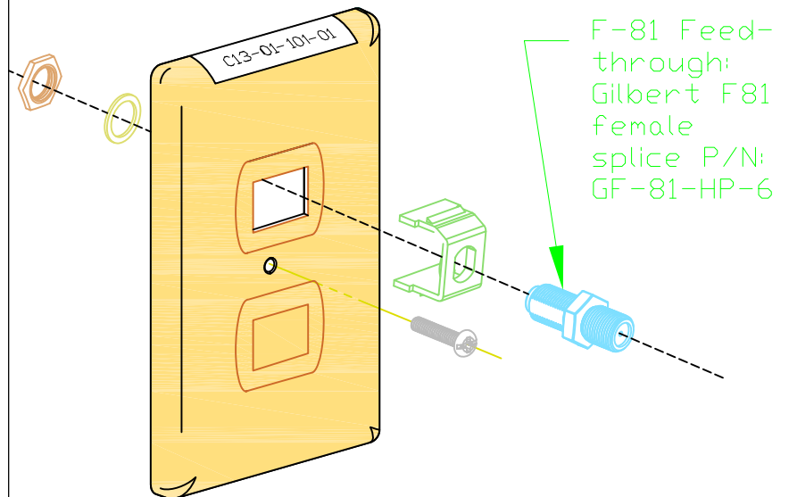
DETAIL No. 7 - CATV Outlet
