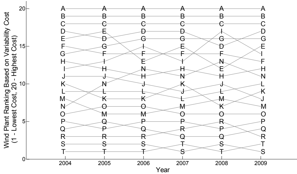
Figure 19 - Change in 2009 wind plant rankings based on variability cost for six different years of ancillary service prices
