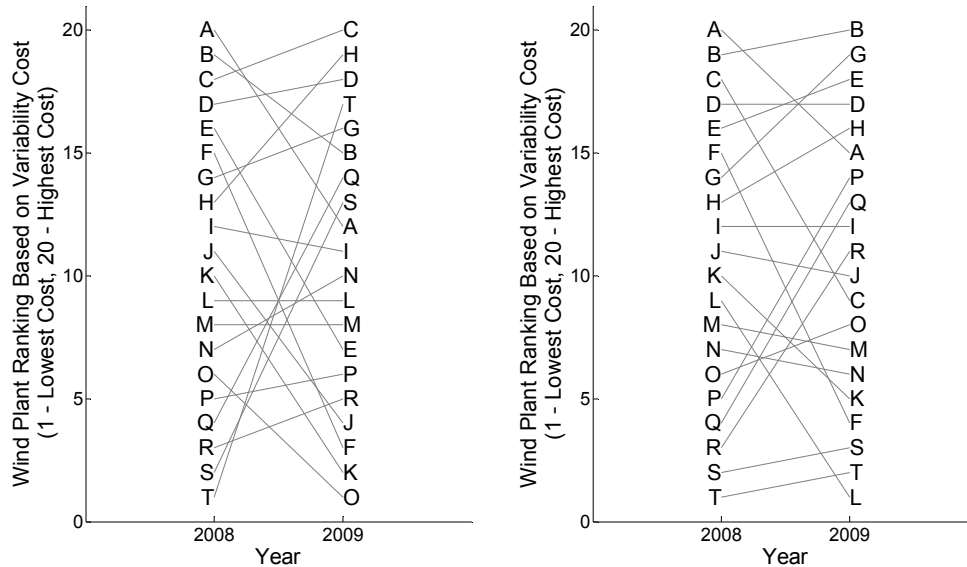
Figure 20 - Change in wind plant rankings when the ancillary price data is held constant. In the left subplot, 2008 ancillary price data was used with 2008 and 2009 wind power data. In the right subplot, 2009 ancillary service prices were used with 2008 and 2009
