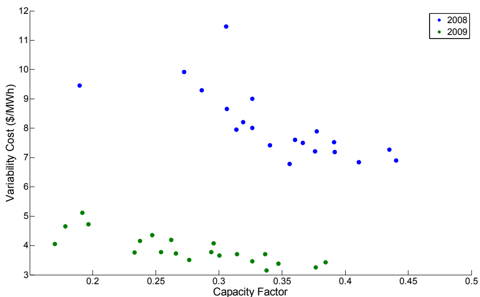
Figure 2 - Estimated variability costs for 20 ERCOT wind plants versus their capacity factors for 2008. The variability cost of wind power decreases as the capacity factor of a wind plant increases.
