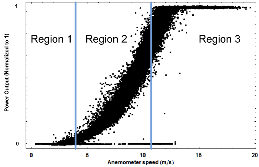
Figure 16 - Actual power curve for a wind turbine
