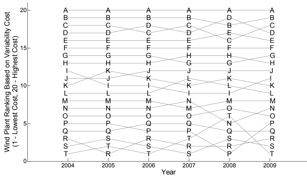
Figure 18 - Change in 2008 wind plant rankings based on variability cost for six different years of ancillary service prices
