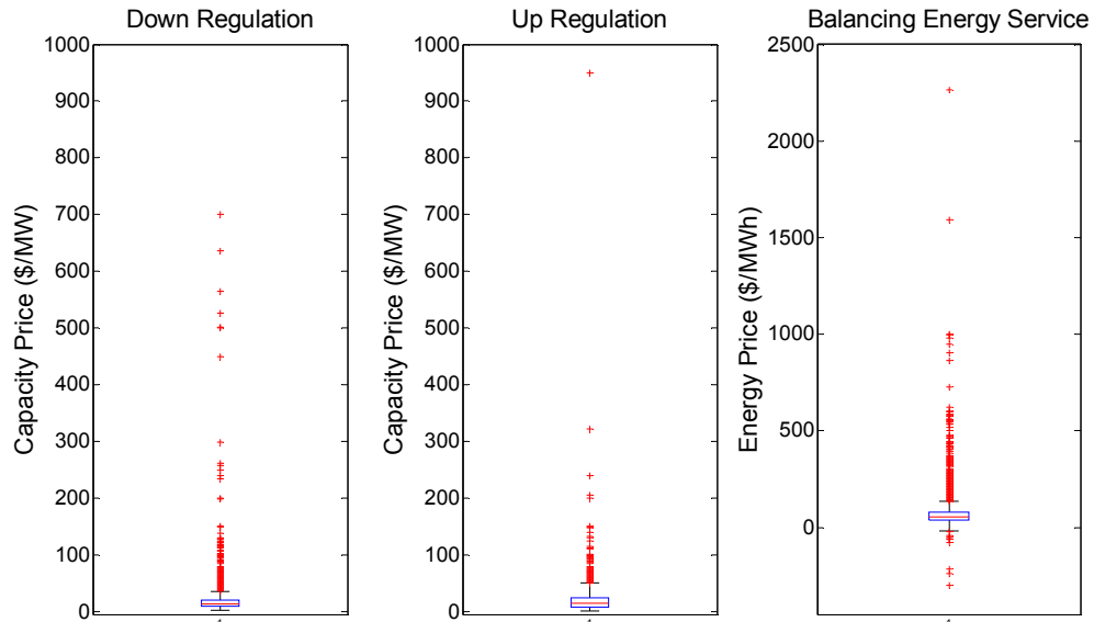
Figure 9 - Box plots for 2005 ERCOT ancillary service prices
