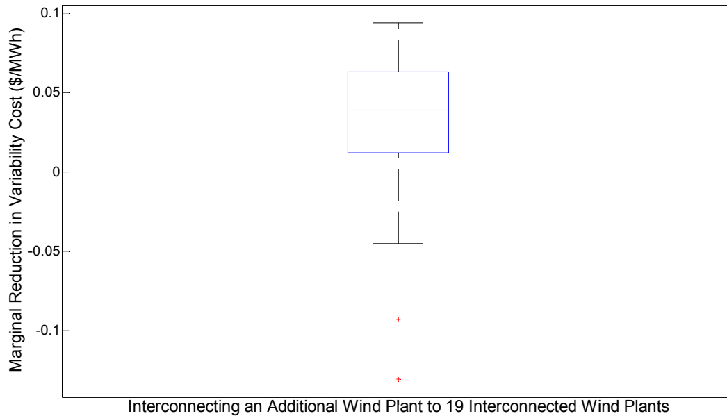
Figure 17 - Box plot of marginal reductions in variability cost for interconnecting a 20th wind plant. All 20 possible cases were estimated.
