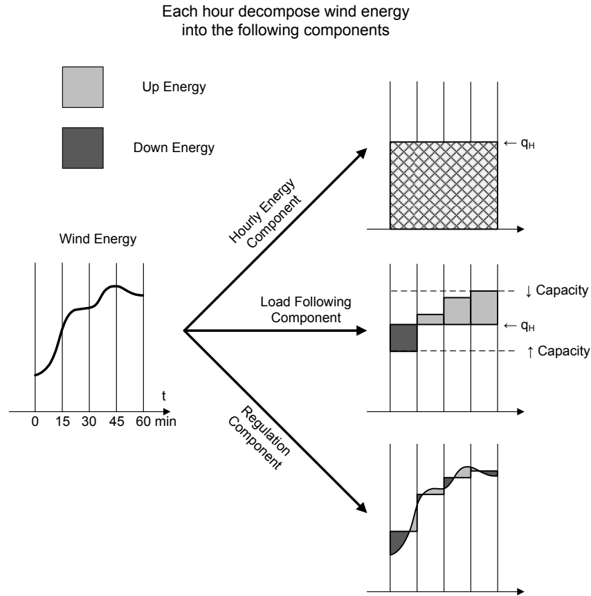
Figure 1 - Conceptual diagram of how we partition wind energy into hourly energy, load following, and regulation components.
