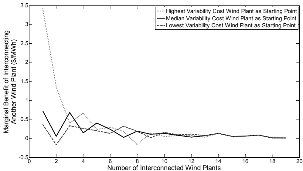
Figure 4 - Marginal benefit of interconnecting an additional wind plant in reducing variability costs. For example, with one wind plant interconnected to a system, the maximum marginal benefit of interconnecting another wind plant is $3.43 per MWh.
