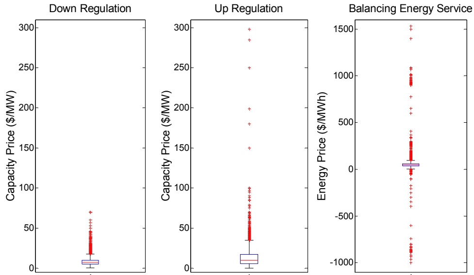
Figure 11 - Box plots for 2007 ERCOT ancillary service prices
