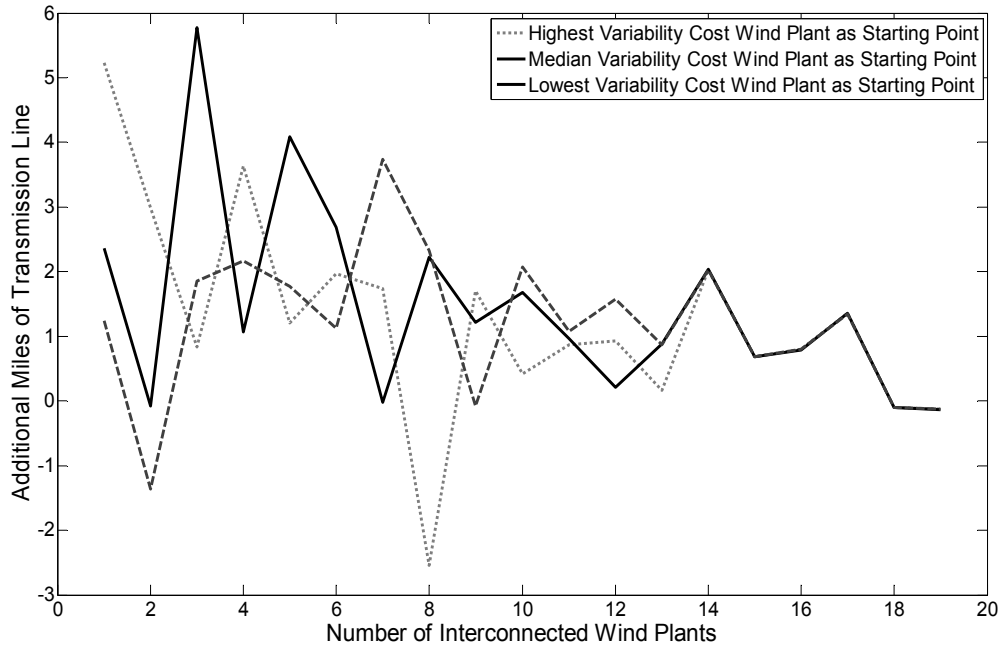
Figure 5 - Marginal benefit of interconnecting an additional wind plant valued in terms of miles ERCOT would be willing to extend a 2GW, 100 mile transmission line.
