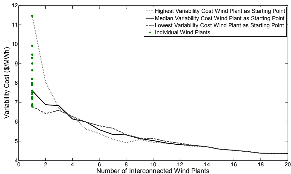
Figure 3 - Variability costs of wind energy decrease as wind plants are interconnected. Interconnecting 20 wind plants together produces a mean savings of $3.76 per MWh compared to the 20 individual ERCOT wind plants (green dots). Only 8 wind plants need to be interconnected to achieve 74% of the reduction in variability cost. Three cases are shown where the highest, median, and lowest variability cost wind plants were used as starting points and the remaining 19 wind plants were interconnected to them based on distance (closest to farthest).
