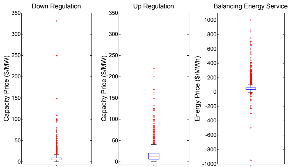
Figure 10 - Box plots for 2006 ERCOT ancillary service prices
