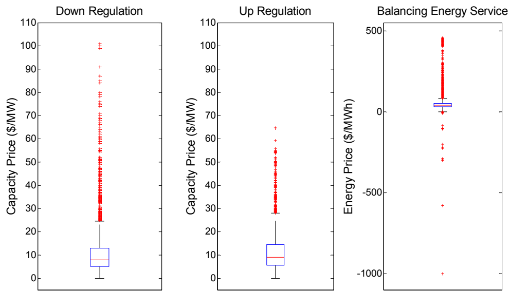
Figure 8 - Box plots for 2004 ERCOT ancillary service prices
