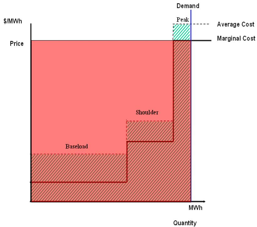
Figure 14: In the uniform-price auction used in U.S. RTO markets, all dispatched generation is paid based on the bid of the marginal generator (in this case, the peaking unit). The total generation cost of serving the load is equal to the amount of load served times the market-clearing
