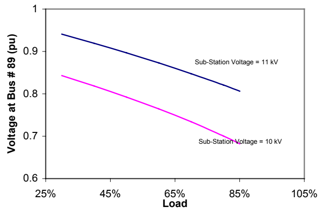
Fig 5. Voltage at Bus # 89 under different loads when the sub-station voltage is 11 kV and 10 kV.
