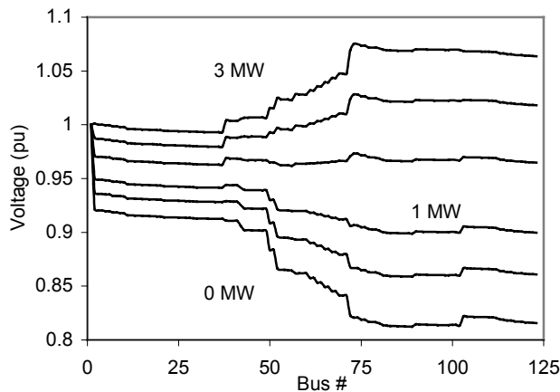
Fig 6. Impact of a decentralized generator placed centrally at Bus # 73 on the voltage profiles. The generator is varied from 0 MW to 3 MW. (On-Line load is 60%, theft 15%, power factor 0.8)
