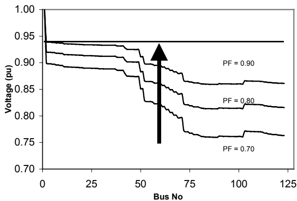
Fig 3: Voltages (pu basis) at different buses in the 128 bus feeder in Tumkur, Karnataka under heavy loads. On-Line load is 75% of the sanctioned load, theft is 15% of on-line load and power factor is varied parametrically between 0.7 – 0.9. The horizontal line is the acceptable voltage of 0.94 pu.
