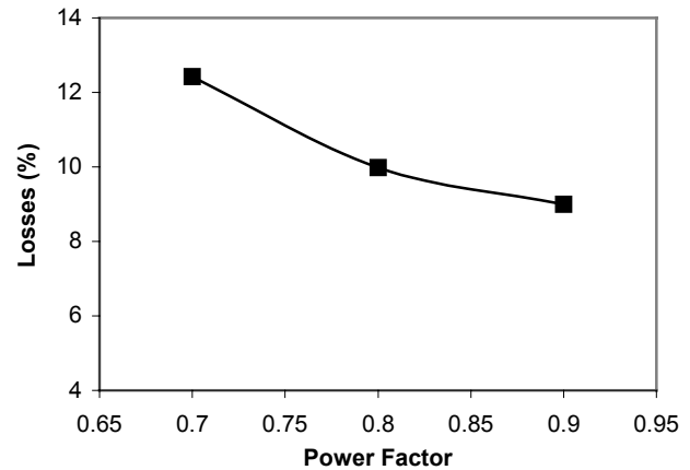
Fig 4. Technical Distribution Losses ( I^2R ) in the feeder under moderate loading of 60% as a function of the overall power factor. The losses are 8% to 12%. Thus the total losses after accounting for theft (15%) are 23% - 27% in just the distribution portion of the network.
