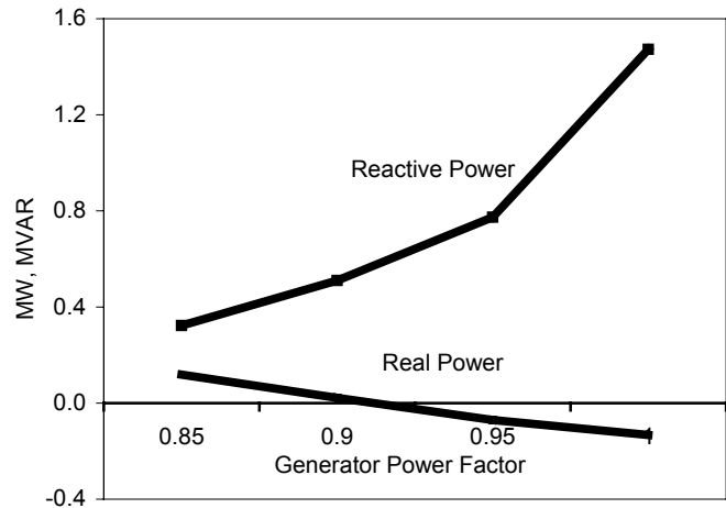
Fig 8. Transactions of real and reactive power with the grid when the power factor of a 3 MVA generator is varied between 0.85 lagging and 1.
