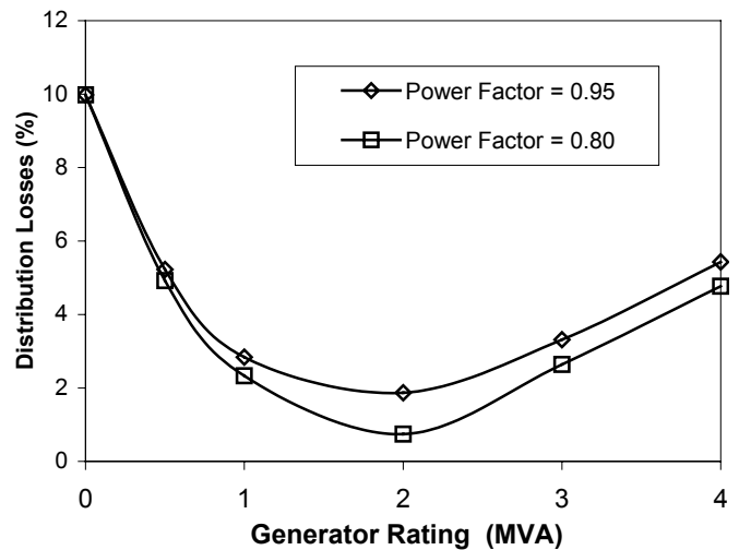
Fig 7. Technical distribution losses for different MVA ratings of the generator (0-4 MVA) and for two generator power factors of 0.80 and 0.95.
