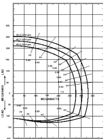
Fig 9. Typical Generator Capability Curve showing the limits of real and reactive power frontiers.
