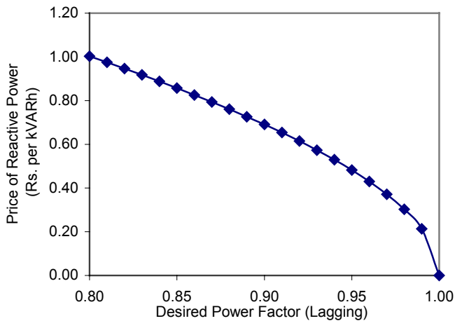
Fig 10. Suggested reactive power pricing (Rs./kVARh) for a 2 MVA generator operating as per the generator capability curve in Fig. 9.
