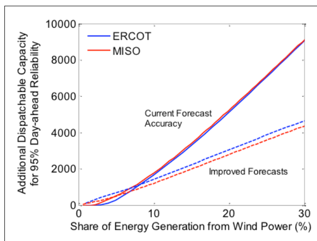
Figure 15: Additional reserve capacity for a range of wind penetration values in ERCOT and MISO. In this figure the horizontal axis is the percentage of load served by wind power. Solid lines assume no change in wind forecast accuracy. Dashed lines show the effect of improved forecasts.
