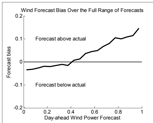
Figure 14: Wind forecast bias as a function of the day-ahead wind forecast in the Electric Reliability Council of Texas (ERCOT) for 2009 and 2010.
