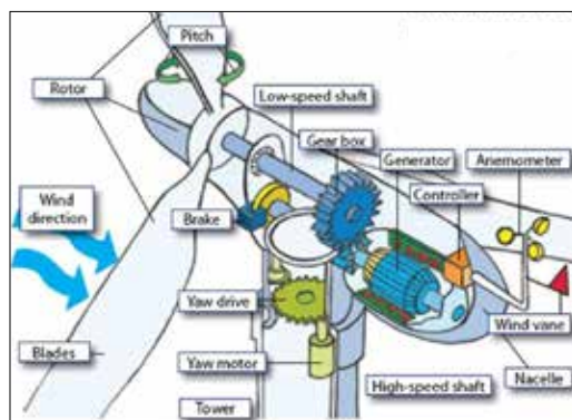
Figure 4: How Does a Wind Turbine Work?
