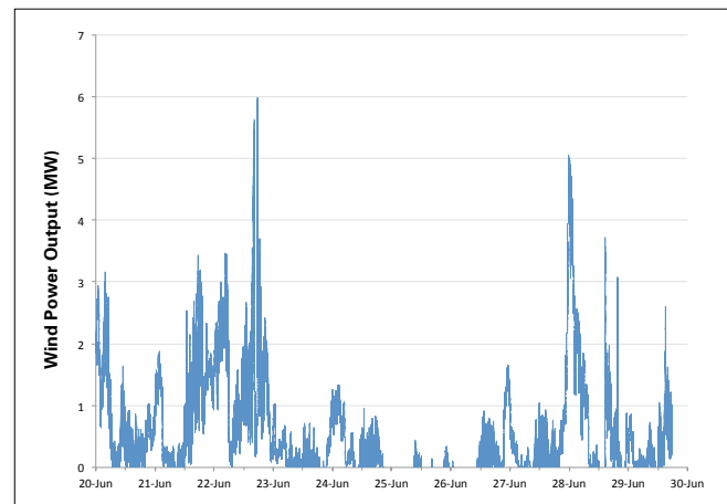
Figure 8: 1-Second Wind Power Output for 10 Days from One Wind Farm.
