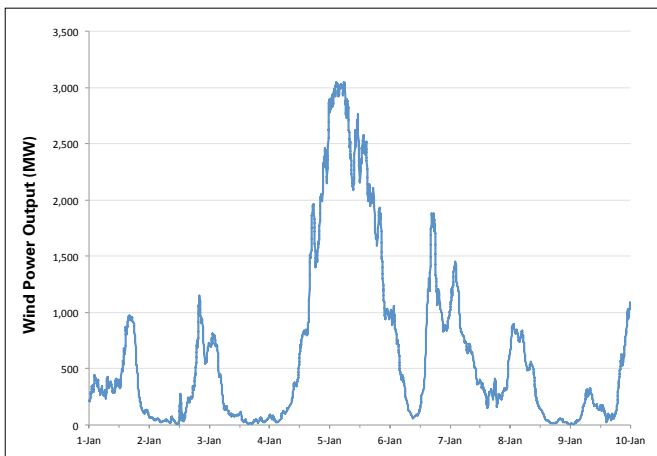
Figure 7: 5-Minute Wind Power Output in BPA, 1/1/2012 to 1/8/2012.
