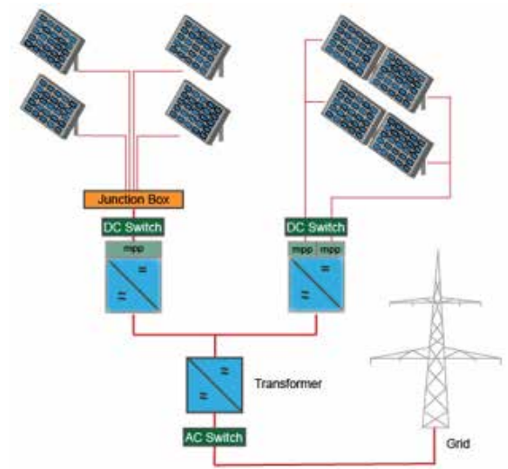
Figure 5b: How Solar Photovoltaic Energy Works
