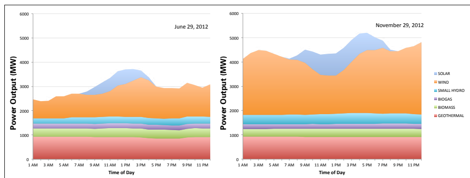
Figure 6: Hourly Renewable Power Output in California for 6/29/2012 and 11/29/2012
