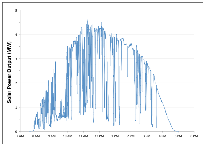
Figure 9: Solar photovoltaic output from a 4.6 MW solar power system in Arizona sampled with 10-second time resolution for the daylight portion of one day.
