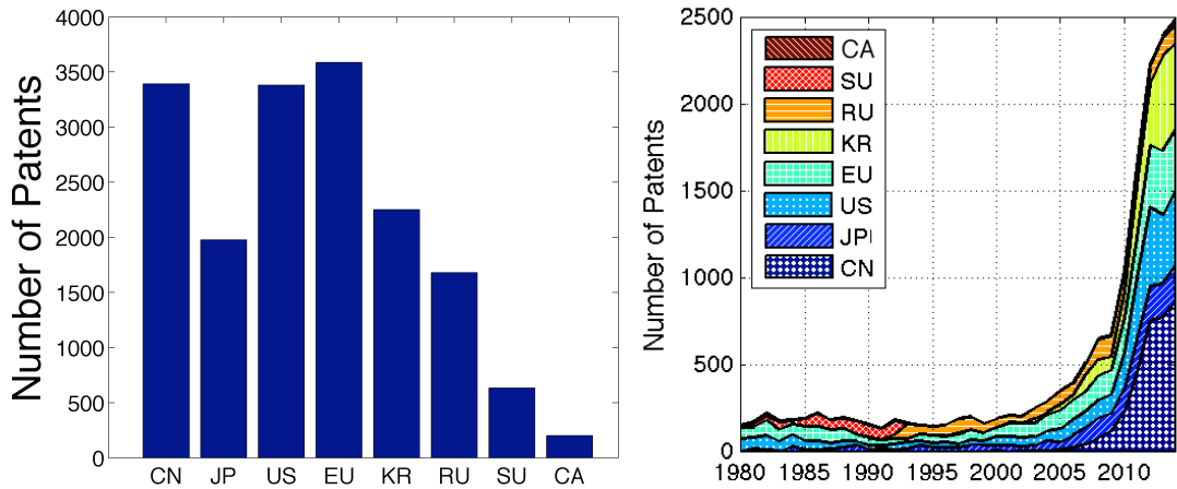
Figure 2.4: Wind power patents granted by all patenting offices: (a) total wind patents from 1980 to 2014 by country/region and (b) wind patents over time by country (China = CN, Japan = JP; United States = US; EU = European Union 15 and EPO member states; South Korea = KR; Russia = RU; Soviet Union = SU; Canada = CA). Data from PATSTAT 2015; plot produced by the authors.
