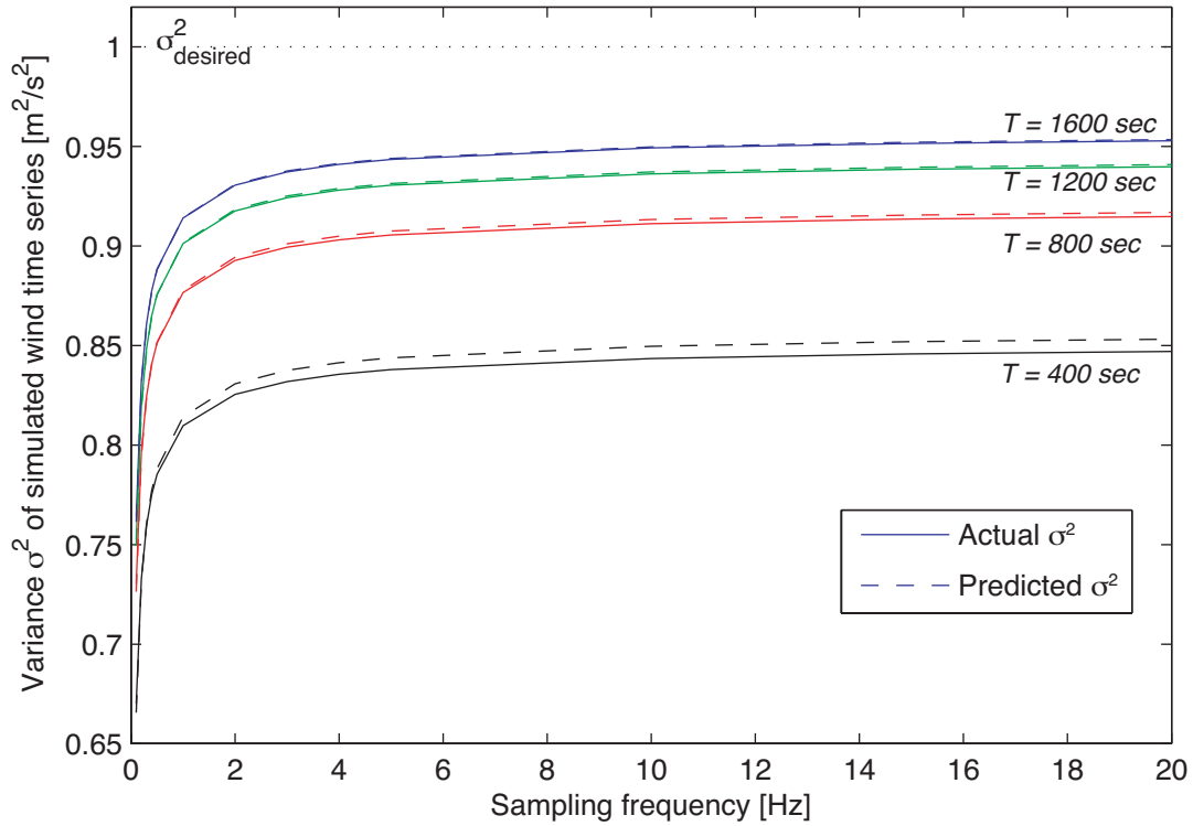
Figure 3.2: This figure plots the actual variance of turbulence simulated with the Kaimal spectrum in equation (3.1) and a variance parameter \sigma^2_{desired} = 1 against the sampling frequency of the simulation. Different curves plot simulations of different lengths. The actual variance is plotted as solid lines and the variance predicted by equation (3.10) is plotted as dotted lines. The turbulence is simulated with Veers method, the Kaimal spectrum from equation (3.1), U = 10 m/s, \sigma^2 = 1 m 2 /s 2 , and z = 65 .
