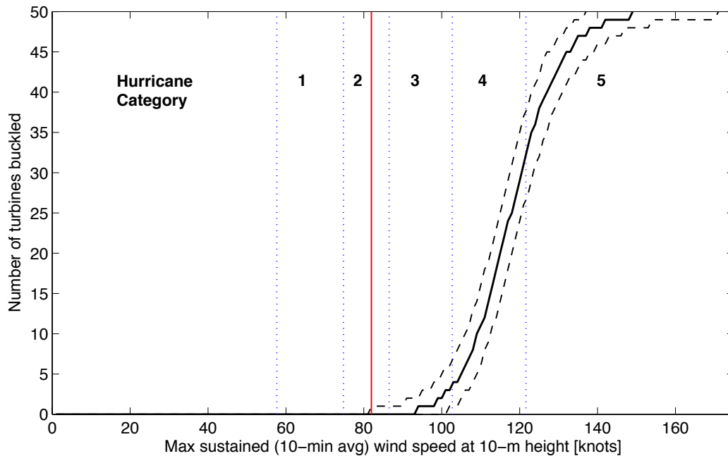
Figure 4.5: Cumulative distribution function of the expected number of turbine towers buckled by a single storm as a function of wind speed. This models a hurricane with a turbulence intensity of 9% in a 50-turbine wind farm of NREL 5-MW turbines (35) that cannot yaw to track the wind. The dashed lines plot the 5th and 95th percentile values and the solid vertical line shows V_{ref} , the design wind speed with a 50-year return period (15) scaled to 10-m height.
