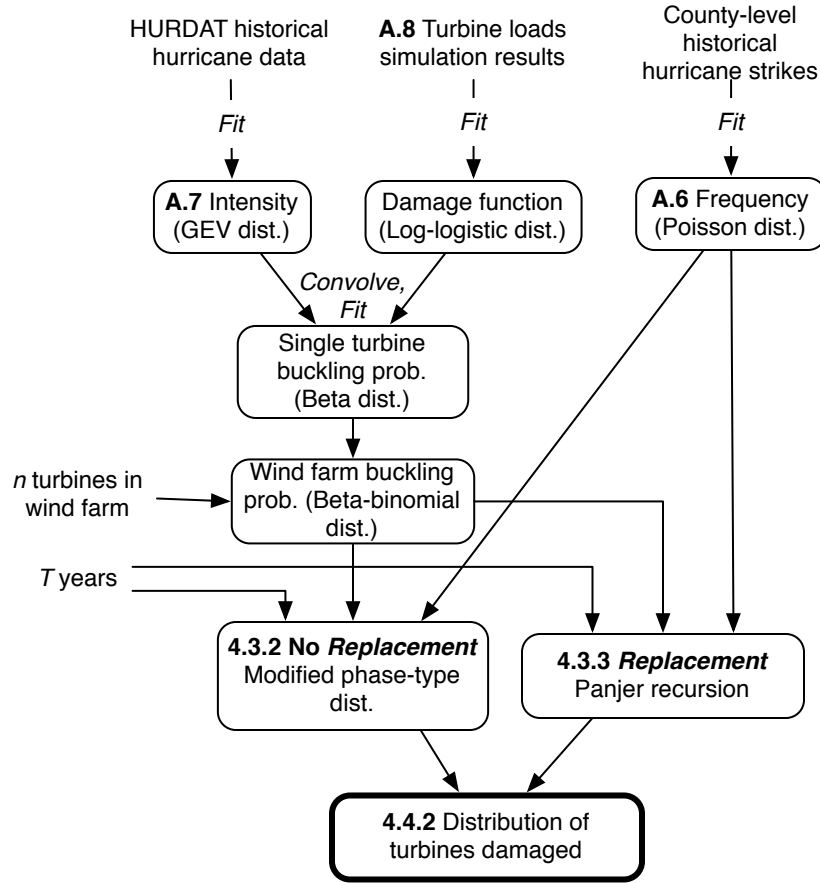
Figure 4.3: Flow chart for calculating the hurricane risk to offshore wind farms using historical hurricanes.
