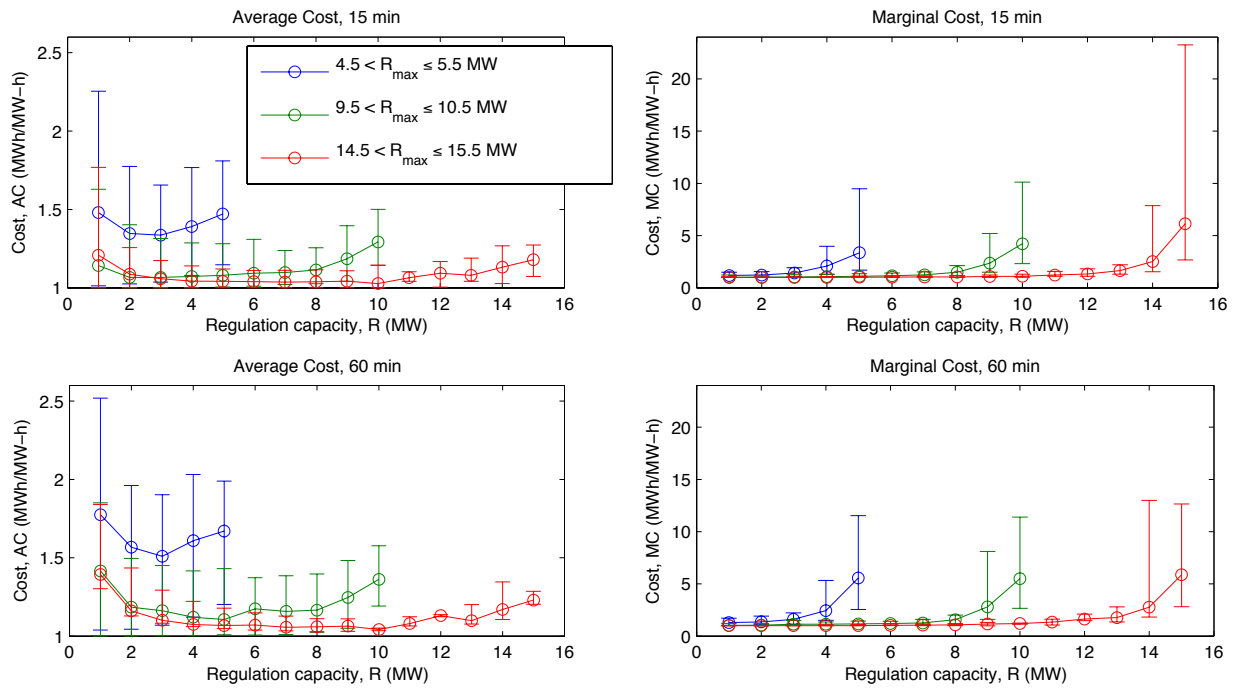
Figure 2.2: The average cost (AC) and marginal costs (MC) of regulation capacity for 15-minute and 60-minute dispatch intervals. Each line represents cost data for dispatch intervals with maximum available regulation capacity in a certain interval described in the figure key. Circles denote the median and error bars show the 5th and 95th percentile costs. These results are calculated for a 100-MW wind farm simulated with wind speed data from west Texas in 2008.
