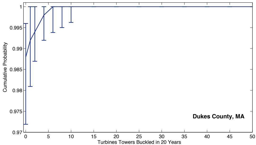
Figure B-2: Cumulative distribution of number of turbine towers buckled in Dukes County, MA by hurricanes in 20 years if buckled towers are not replaced. Solid lines plot the distribution for the cast that turbines cannot yaw. Results for yawing turbines are not shown because the risks are too small to calculate with the method in this paper.
