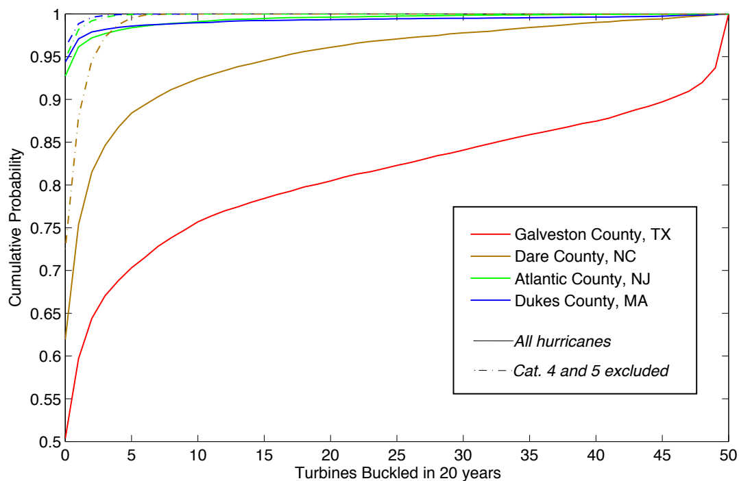
Figure A-2: CDF of the number of turbine towers buckled in 20 years without replacement; turbines cannot yaw to track the wind. Solid lines plot the distribution including all hurricanes, and dotted lines plot the distribution with category 4 and 5 hurricanes excluded.
