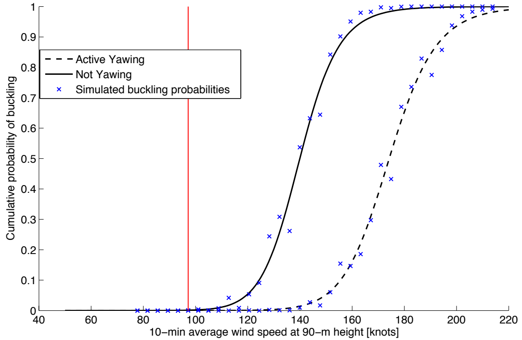
Figure A-7: Log-logistic functions fitted to probability of tower buckling as a function of wind speed. The vertical red line at 95 knots plots the 10-minute sustained wind speed with a 50-year return period used to design Class I wind turbines in the IEC 61400-3 standard.
