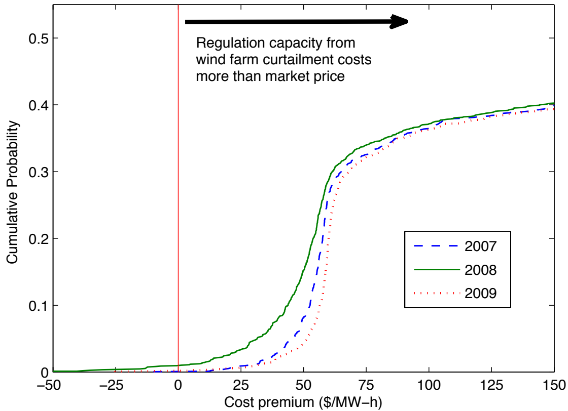
Figure 2.3: A CDF of the cost premium for regulation capacity from a curtailed wind farm, as compared to ERCOT market prices for upregulation. The curtailed wind farm can provide upregulation at less than the market price in fewer than 1% of the 1440 1-hour periods studied and at any price in approximately 45% of the periods studied. We assume an opportunity cost for curtailing the wind farm of $62/MWh.
