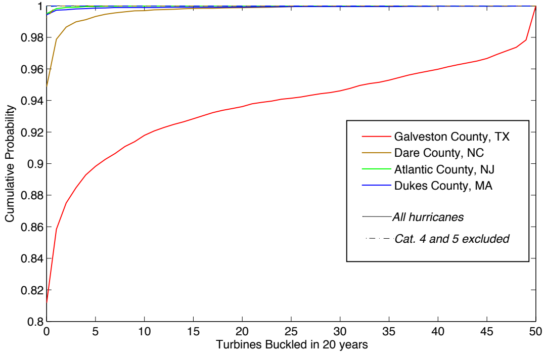
Figure A-3: CDF of the number of turbine towers buckled in 20 years without replacement; turbines can actively yaw to track the wind. Solid lines plot the distribution including all hurricanes, and dotted lines plot the distribution with category 4 and 5 hurricanes excluded.
