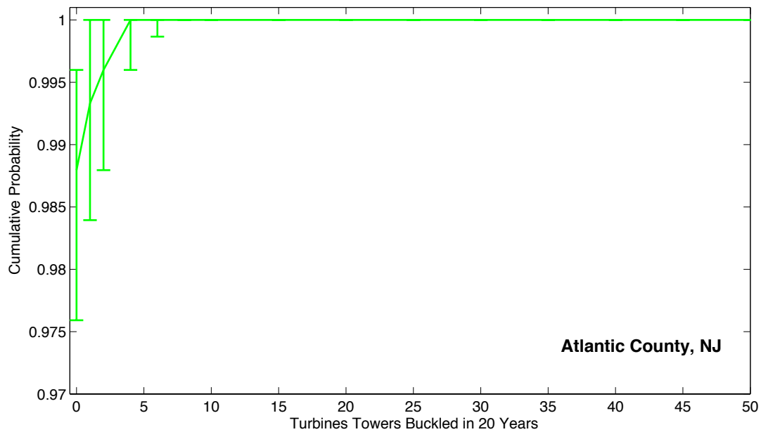
Figure B-1: Cumulative distribution of number of turbine towers buckled in Atlantic County, NJ by hurricanes in 20 years if buckled towers are not replaced. Solid lines plot the distribution for the cast that turbines cannot yaw. Results for yawing turbines are not shown because the risks are too small to calculate with the method in this paper.
