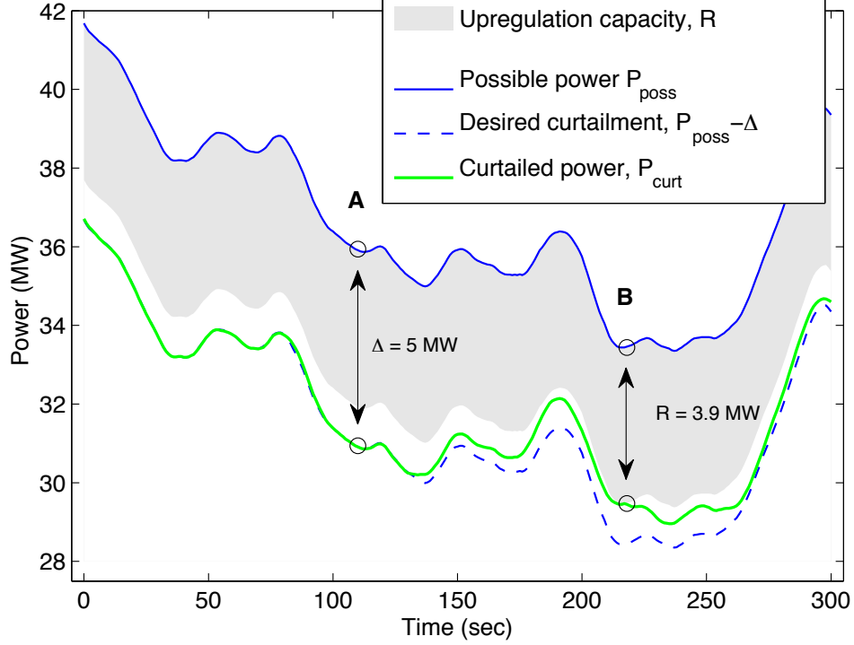
Figure 2.1: Method for calculating the available regulation capacity. In this example, the 100 MW-capacity wind farm is curtailed by \Delta = 5 MW, but the available regulation capacity R(k | \Delta) is 3.9 MW. R(k | \Delta) is the largest curtailment that can be maintained through the entire dispatch interval T , i.e. the smallest difference between the uncurtailed and curtailed power outputs of the wind farm. The limiting condition is shown at point B. Point A shows an example of the turbines tracking their power limit setpoints perfectly—the actual curtailed power is 5 MW less than the uncurtailed power, as it is commanded to be.
