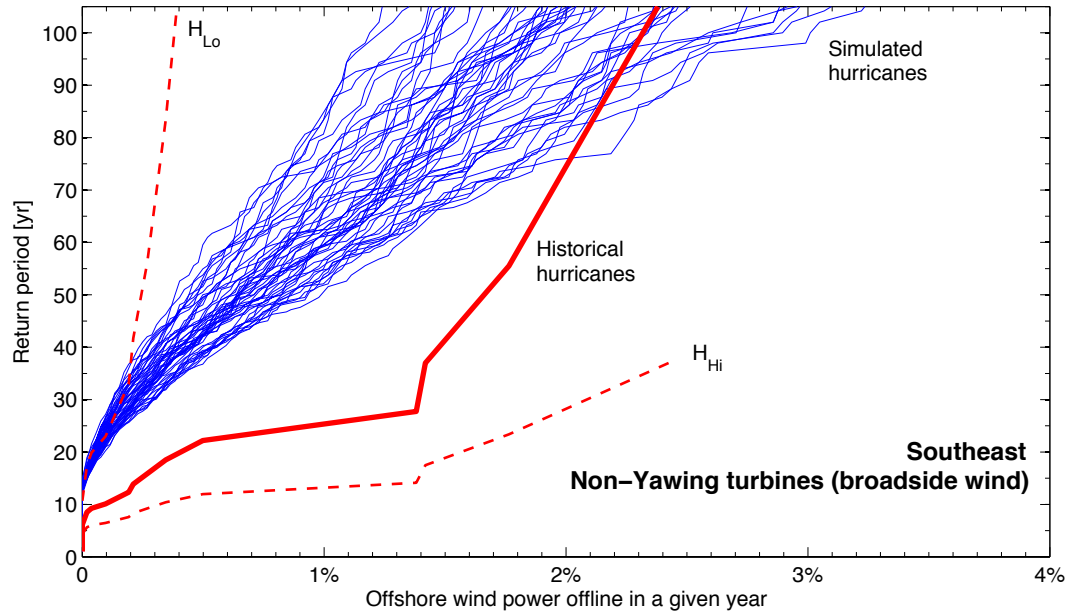
Figure 5.6: Return period for fraction of wind power offline due to hurricane damage in the Southeast (GA, SC, NC), assuming turbines are placed in all locations described above (total capacity of 104 GW) and the turbines cannot yaw. We do not show the results for yawing turbines because the risks are negligible. Each of the “Simulated hurricanes” lines represents one of the fifty 5,000-year periods of simulated hurricanes. The “Historical hurricane” line represents risk calculated from the historical hurricane record (1900 - 2011) and “H Lo ” and “H Hi ” represent the lower and upper confidence bounds for the historically-based estimates.
