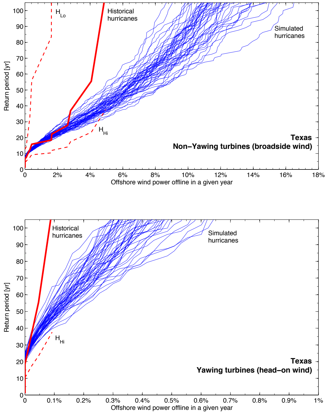
Figure 5.5: Return period for fraction of wind power offline due to hurricane damage in the Texas, assuming turbines are placed in all locations described above (total capacity of 87 GW). The top plot gives risks for non-yawing turbines; the bottom gives risks for yawing turbines. Each of the “Simulated hurricanes” lines represents one of the fifty 5,000-year periods of simulated hurricanes. The “Historical hurricane” line represents risk calculated from the historical hurricane record (1900 - 2011) and “ H_{Lo} ” and “ H_{Hi} ” represent the lower and upper confidence bounds for the historically-based estimates.
