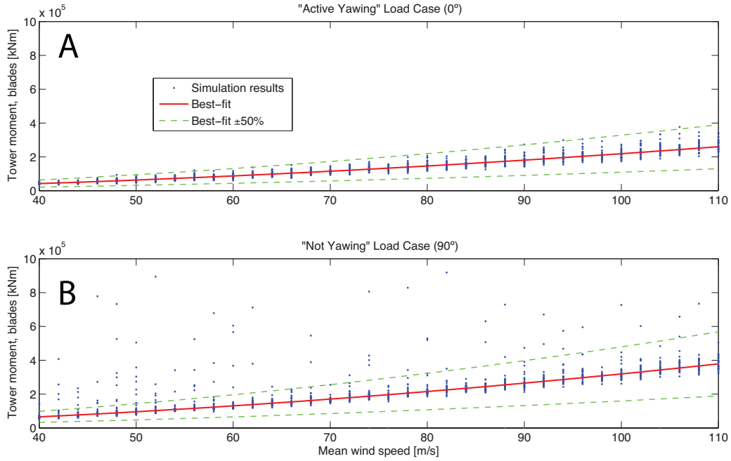
Figure A-10: The method for excluding anomalous simulation results for maximum tower bending moment. The red line is a robust linear best-fit to the data and the green dashed lines are 0.5 and 1.5 times the best-fit line. Data outside the green dashed lines are excluded.
