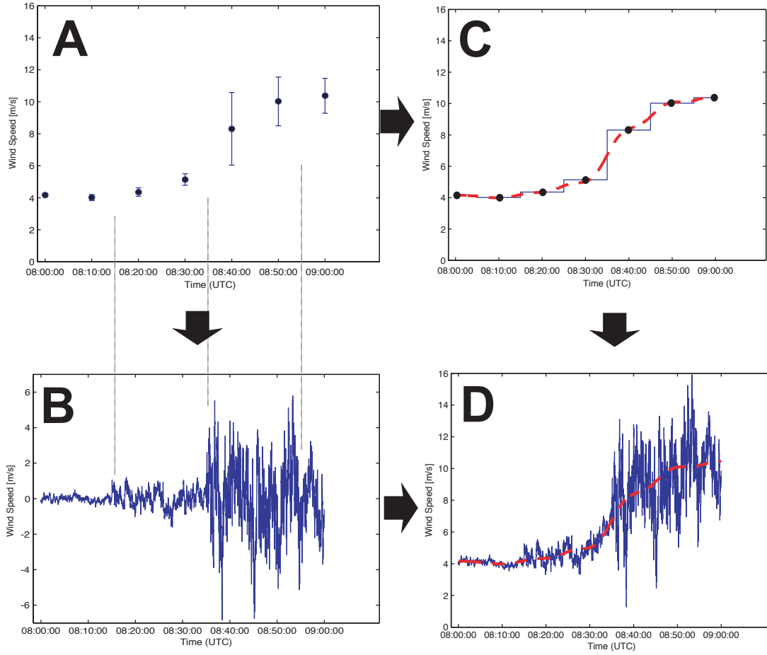
Figure 3.1: Procedure for generating wind speed time series from a hybrid of measured and simulated data. (A) Wind speed mean and variance measured for a long period T_{input} are used as parameters to generate zero-mean turbulence in (B). The mean wind speeds in (A) are re-sampled at a higher rate f_{output} and smoothed by a low-pass filter in (C). The hybrid wind speed time series in (D) is the sum of (B) and (C).
