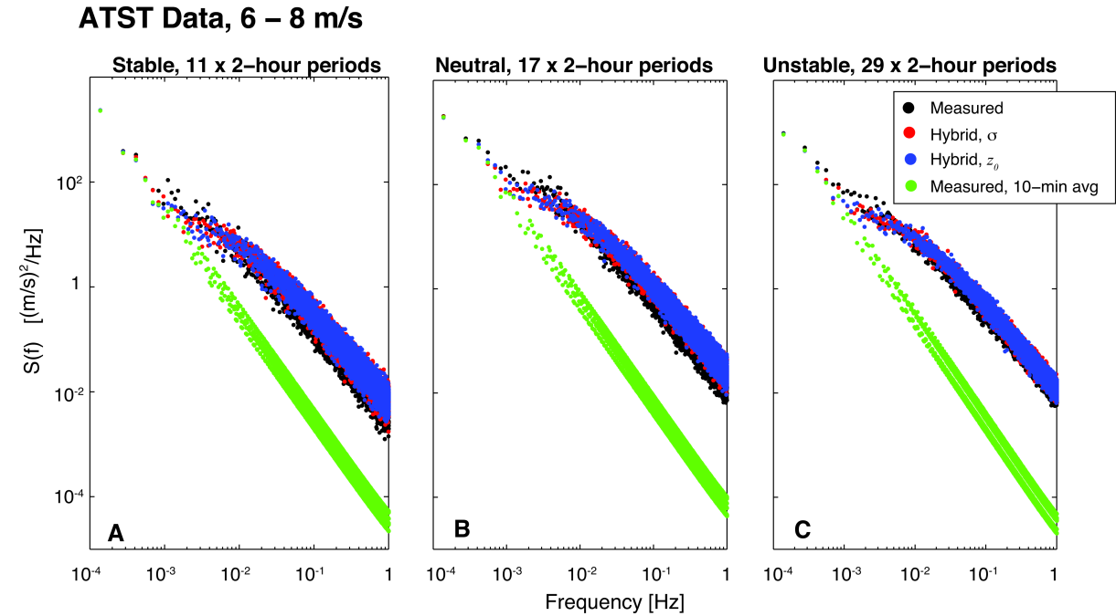
Figure 3.4: A comparison of Power Spectral Densities (PSD) of measured wind data, both variants of hybrid wind speed data, and measured 10-minute average data from the ATST field site for 6 – 8 m/s mean wind speed. Each PSD is the segment average of the PSDs all 2-hour segments of data in the specified mean wind speed range (see description in text). Data from stable conditions ( 0.01 < 1/L < 0.15 ) are plotted in (A), neutral conditions ( -0.03 < 1/L < 0.01 ) are plotted in (B), and unstable conditions ( -0.15 < 1/L < -0.03 ) in (C). We plot the spectral only to 2 Hz because we decimate (low-pass filter and down-sample) the measured data to 5 Hz, but the low-pass filtering attenuates the spectra of the measured data above 2 Hz.
