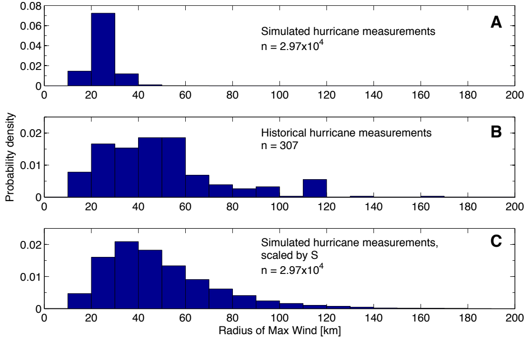
Figure 5.3: Histogram of radius of maximum winds for hurricanes within 200 km of the continental U.S. coast. The distribution of r_{\max} in (C), has been scaled by a lognormal distribution described in Section 5.2.6 to match the distribution of r_{\max} for historical hurricanes in (B) better than the r_{\max} calculated by Emanuel's CHIPS model shown in (A).
