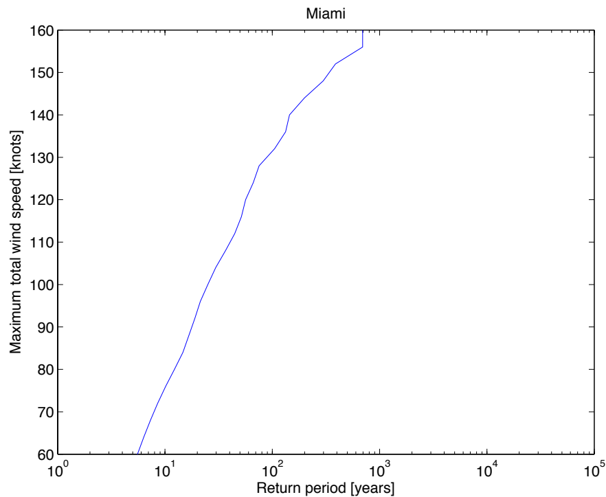
Figure B-7: Return periods for maximum total wind speeds within 100 km of Miami, calculated from the simulated hurricanes described in the body of the paper.
