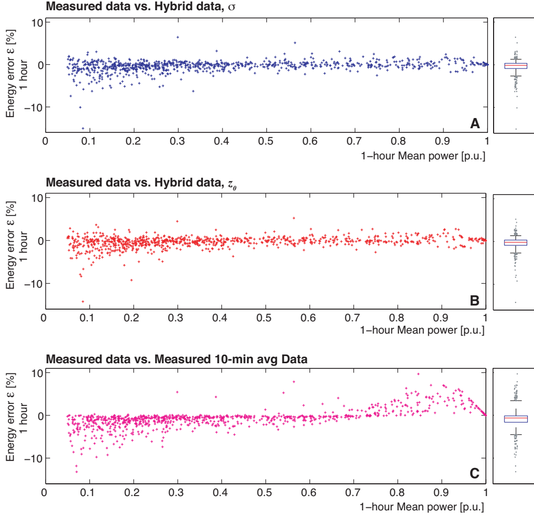
Figure 3.5: The plots on the left show percent difference in energy production \epsilon between a turbine simulated with empirical wind data and hybrid wind data, plotted against per-unit (p.u.) mean power. (A) compares measured data to hybrid data created with equation ( 3.1 ), (B) compares measured data to hybrid data created with equation ( 3.2 ), and (C) compares measured data to 10-minute average measured data. The boxplots on the right plot the mean (center line), 25th and 75th percentile values (bottom and top of box), and the 5th and 95th percentiles (bottom and top “whiskers”) of the same data [40].
