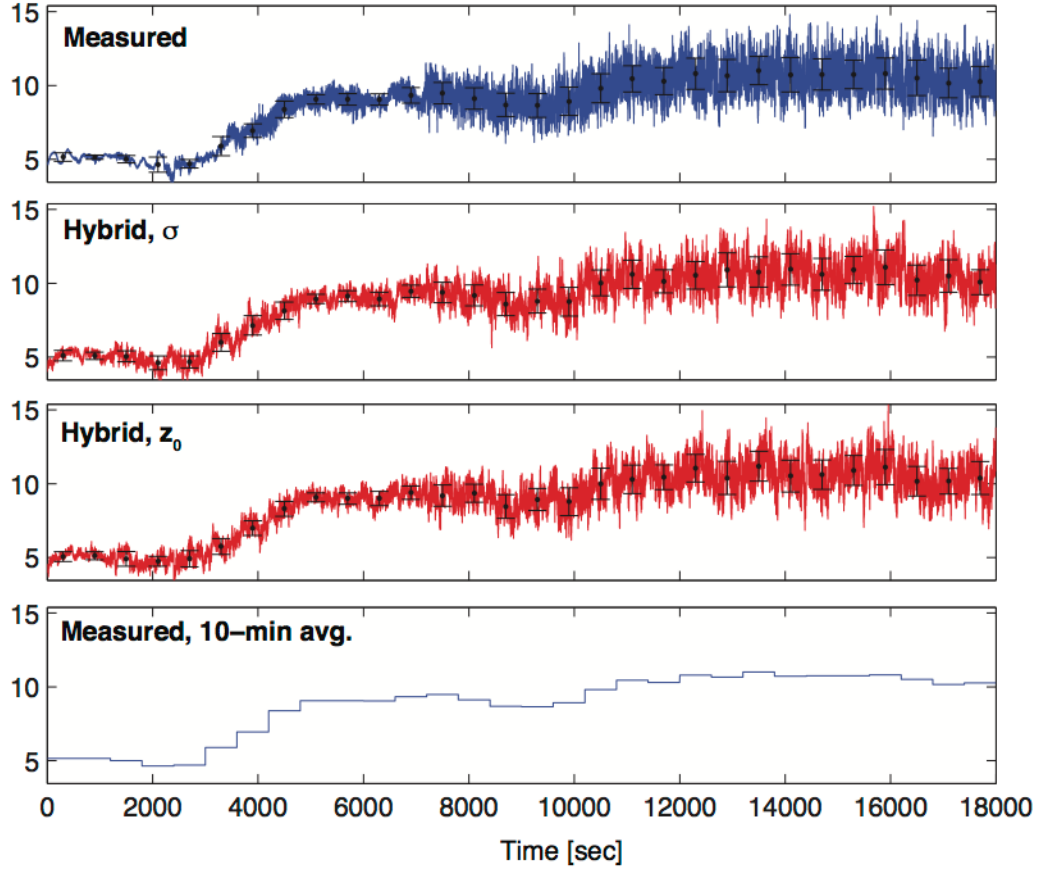
Figure 3.3: A comparison of measured wind speed data (“Measured”), hybrid wind speed data generated with empirical mean and variance statistics (“Hybrid, \sigma ”), hybrid wind speed data generated with empirical mean statistics and estimated surface roughness length (“Hybrid, z_0 ”), and empirical mean statistics (“Measured, 10-min avg.”). These data are representative of the close match between hybrid wind speed data and measured data with similar statistical properties. These plots show 4 hours of data from the CASES99 experiment beginning at 20:00:00 October 28, 1999 (stable atmospheric conditions). The hybrid and “Measured, 10-min avg.” data are generated using 10-minute statistics derived from the “Measured” data.
