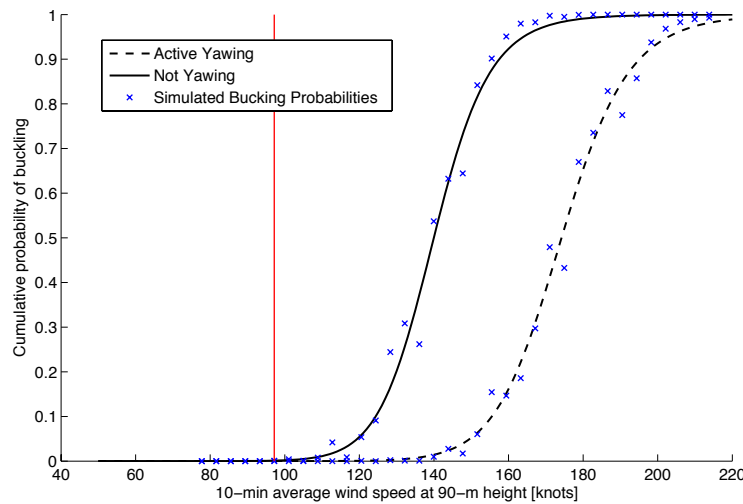
Figure 5.4: Log-logistic functions fitted to probability of tower buckling as a function of wind speed. The vertical red line at 95 knots is the 10-minute sustained wind speed with a 50-year return period used to design Class I wind turbines in the IEC 61400-3 standard.
