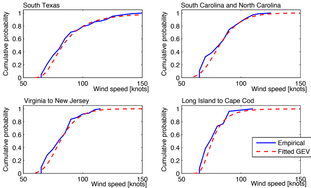
Figure A-6: Comparison of empirical CDFs for maximum hurricane wind speed in the regions we examine and the GEV distributions fitted to those data.
