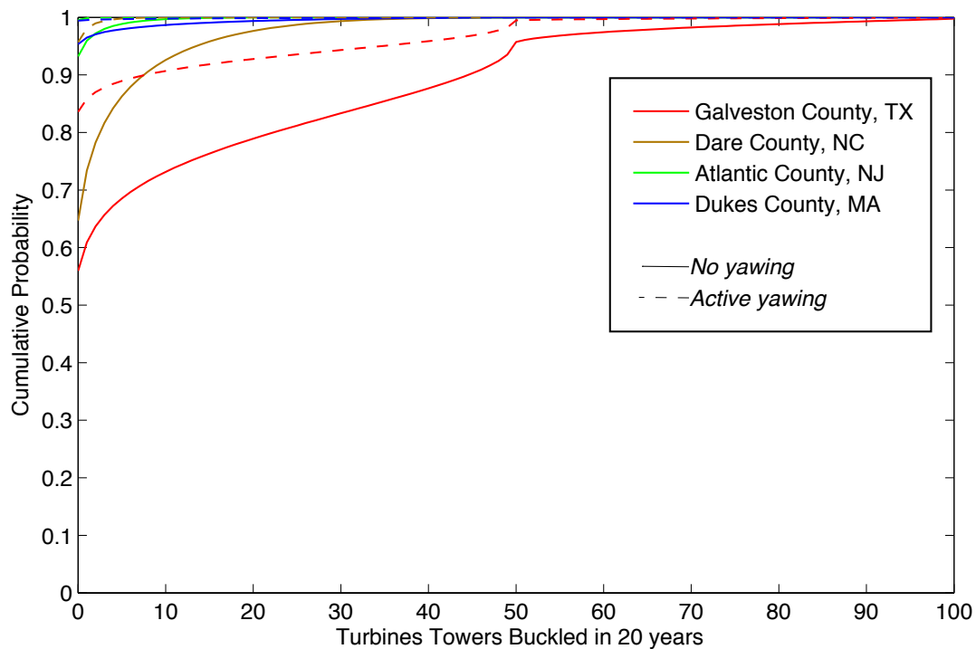
Figure A-1: Cumulative distribution of the number of towers in a 50-turbine wind farm buckled in 20 years if buckled towers are replaced after each storm if they buckle. Dashed lines plot the distribution for the case that turbines can yaw to track the wind direction, and solid lines plot the distribution for the case that turbines cannot yaw.
