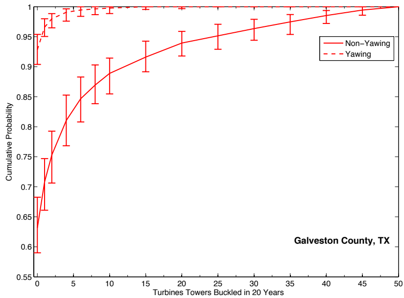
Figure 5.9: Cumulative distribution of number of turbine towers buckled in Galveston County, TX by hurricanes in 20 years if buckled towers are not replaced. Dashed lines plot the distribution for the case that the turbines can yaw to track the wind direction, and solid lines plot the distribution for the cast that turbines cannot yaw.
