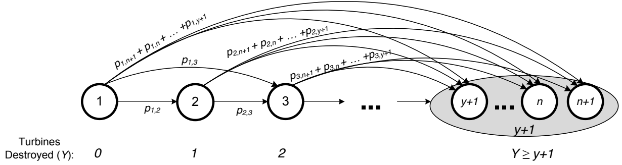
Figure 4.4: The Markov Chain used to calculate the probability that the number of turbine towers buckled is less than or equal to y . We define the absorbing state as all the states where Y_{no\ rep} \geq y+1 .
