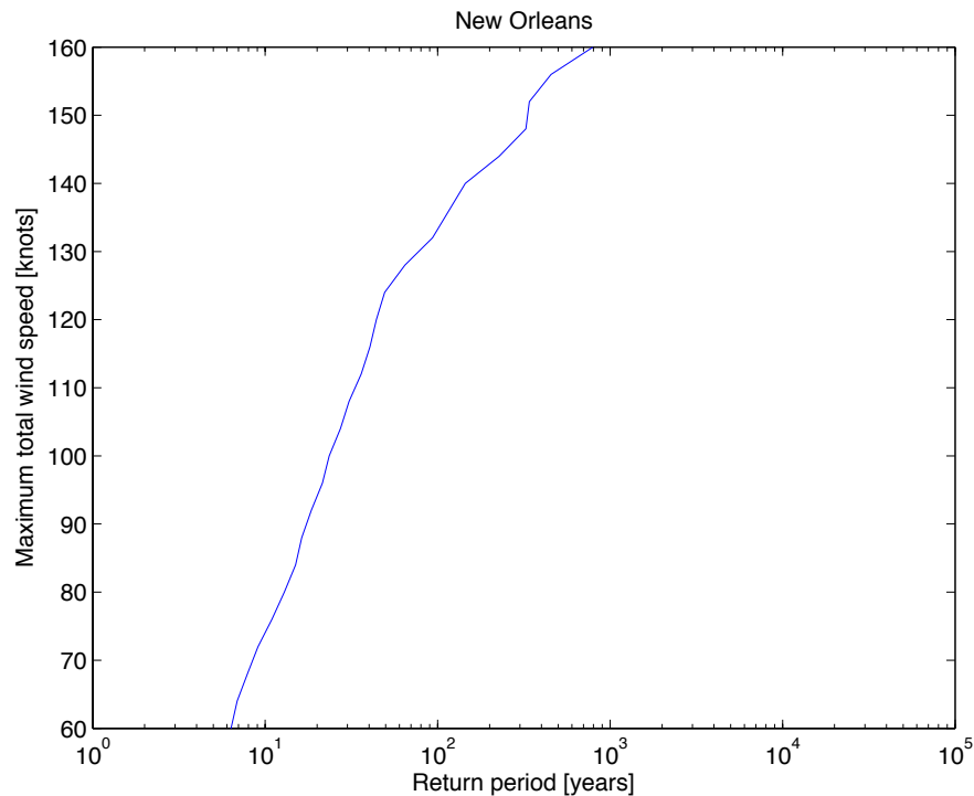
Figure B-6: Return periods for maximum total wind speeds within 100 km of New Orleans, calculated from the simulated hurricanes described in the body of the paper.
