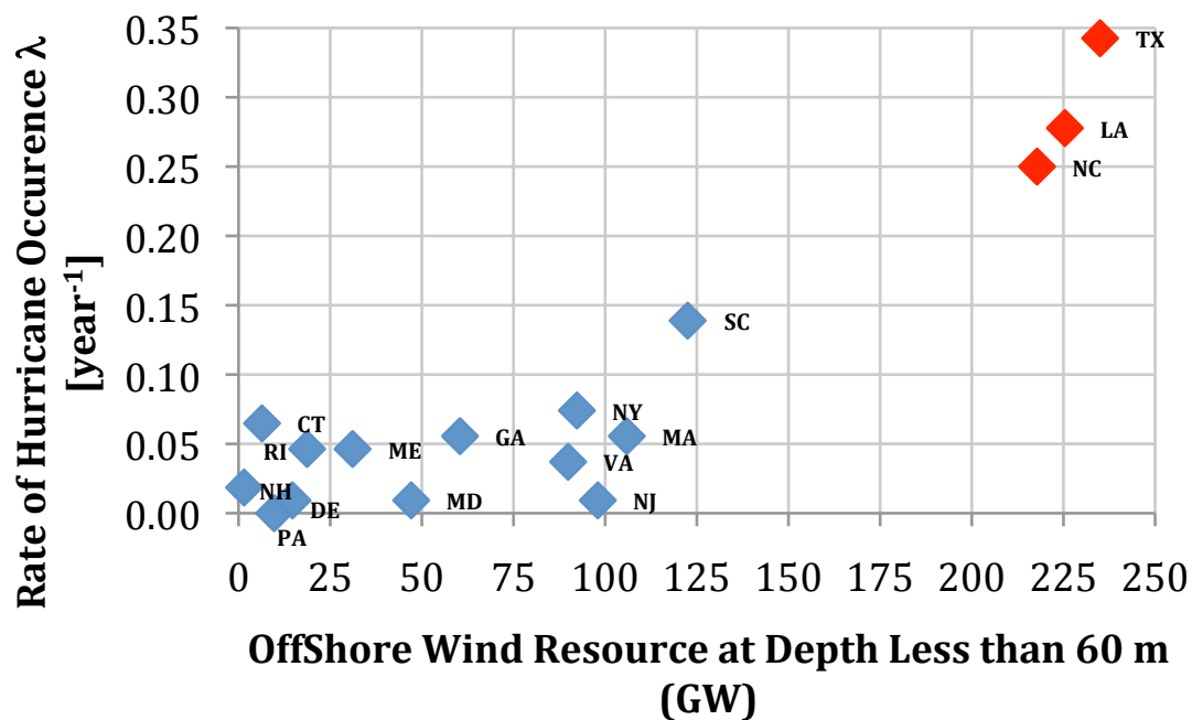
Figure 4.8: Resource vs. Hurricane Occurrence Rate \lambda [year -1 ]. Texas, Louisiana, and North Carolina are shown in red because the annual rate of hurricane occurrence in those states is significantly higher than in the other states considered.
