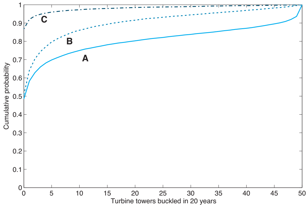
Figure 4.2: Cumulative distribution of the number of turbine towers in a 50-turbine wind at 29.15°N, 94.66°W buckled in 20 years if buckled towers are not replaced and there is no active yawing. The original results for Galveston published in Figure 2 of our paper are shown in (A). Results using the correction for 1 – average wind speeds are plotted in (B). Results using that correction and a wind field model are shown in (C).
