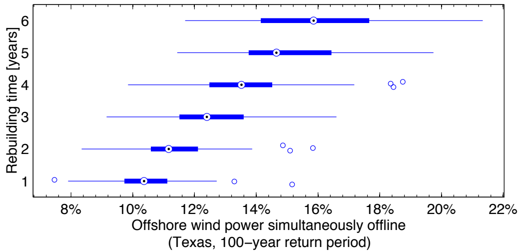
Figure 5.7: Sensitivity of results to rebuilding time. These results are the percentage of Texas offshore wind power simultaneously offline with a 100-year return period. The boxes represent the 25th and 75th percentiles of the simulation results, the whiskers represent the maximum extent of the simulated predictions not classed as outliers, and circles are the outliers.
