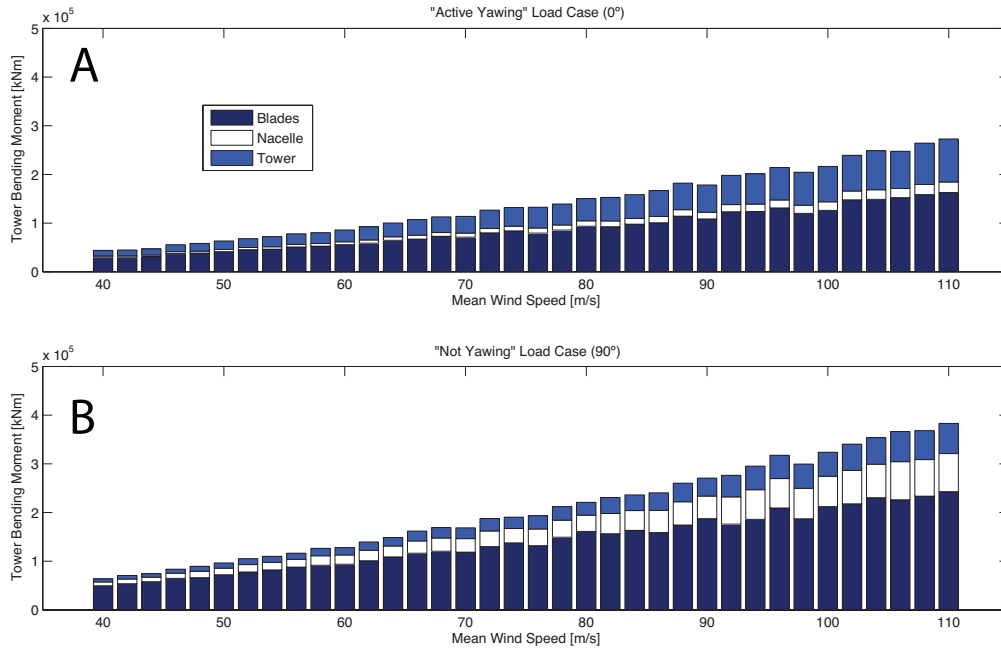
Figure A-9: Magnitude of bending moment on the tower base vs. 10-min mean wind speed. The “Blades” component of the moment is simulated using the NREL FAST software. The “Nacelle” component is calculated using [A8] the “Tower” component is calculated using [A10].
