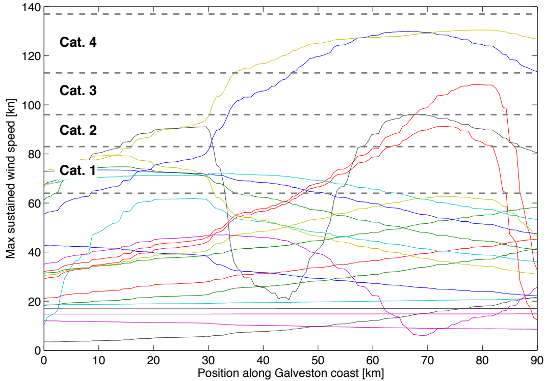
Figure 4.1: Wind profiles at landfall of all hurricanes making landfall in or near Galveston County, TX, 1900-2008.
