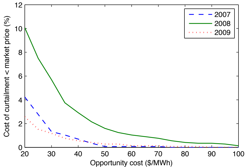
Figure 2.4: Cost-effectiveness of wind farm curtailment for upregulation as a function of opportunity cost of curtailment. As the opportunity cost of curtailment increases, upregulation from curtailment is cheaper than the market price for curtailment in fewer 1-hour dispatch intervals.
