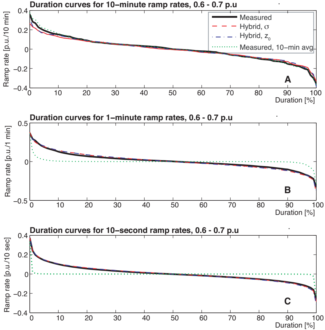
Figure 3.6: A comparison of the distribution (percentiles) of power ramp rates for a simulated turbine driven by measured wind data. All plots show changes in power starting in the range 0.6 – 0.7 per-unit (p.u.); (A) shows the distribution of 10-minute ramp rates, (B) the distribution of 1-minute ramp rates, and (C) the distribution of 10-second ramp rates. The hybrid data are nearly indistinguishable from the measured data, especially for 1-minute and 10-second ramp rates.
