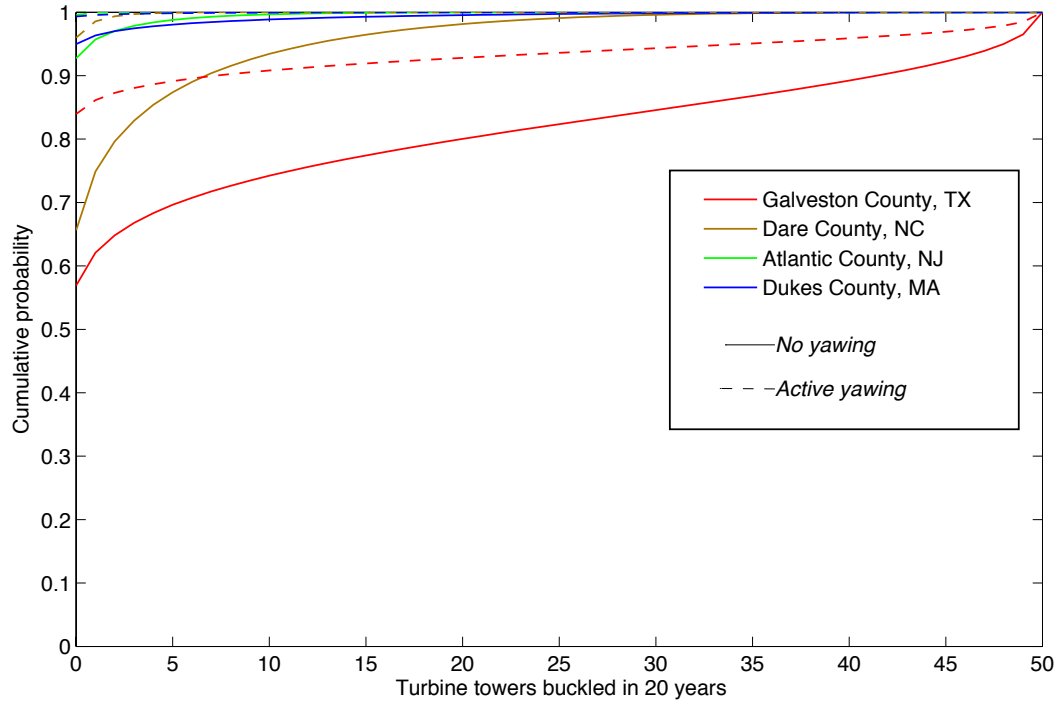
Figure 4.6: Cumulative distribution of the number of turbine towers in a 50-turbine wind farm buckled in 20 years if buckled towers are not replaced. Dashed lines plot the distribution for the case that turbines can yaw to track the wind direction, and solid lines plot the distribution for the case that turbines cannot yaw.
