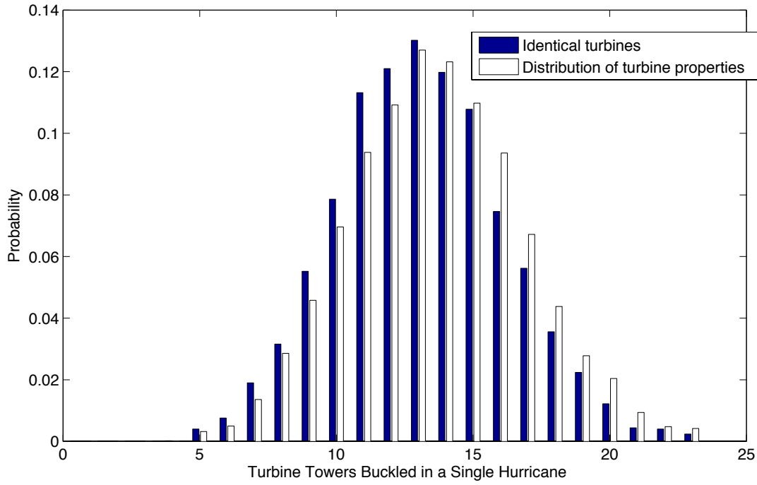
Figure A-11: Distribution of number of turbine towers buckled in a single hurricane a mean wind speed of 70 m/s (136 knots). Blue bars plot results for the case used in our paper, where buckling probabilities are identical for all turbines. White bars plot results for the case where the resistance to buckling of each tower is drawn randomly from the distribution given in (A 11).
