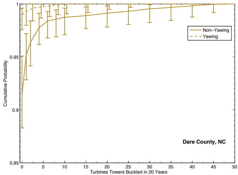
Figure 5.10: Cumulative distribution of number of turbine towers buckled in Dare County, NC by hurricanes in 20 years if buckled towers are not replaced. Dashed lines plot the distribution for the case that the turbines can yaw to track the wind direction, and solid lines plot the distribution for the cast that turbines cannot yaw.
