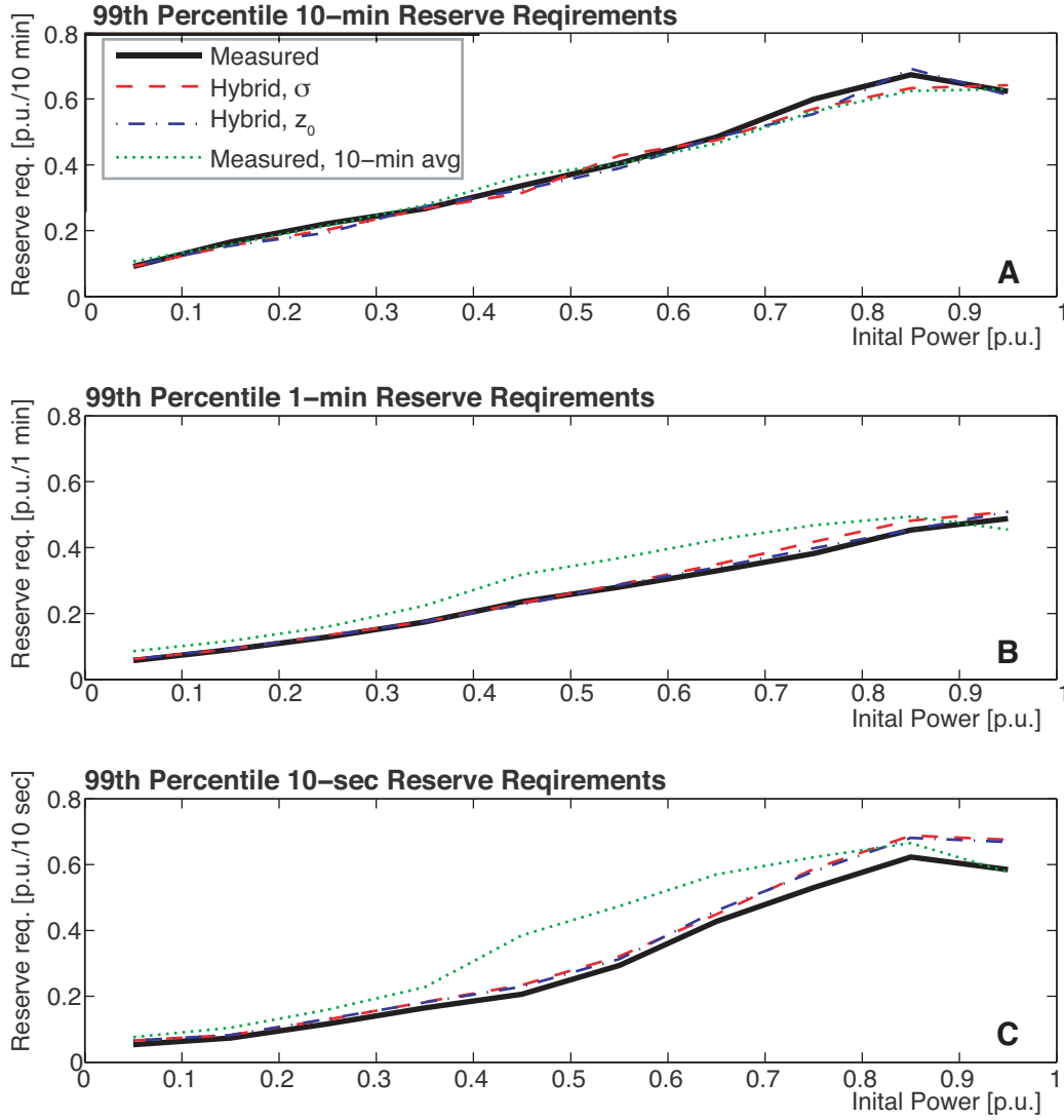
Figure 3.8: The extreme (99th percentile) reserve requirements for a simulated turbine driven by measured and hybrid wind data. Each plot shows the extreme reserve requirement as a function of the initial power (power output at the start of ramping). (A) shows the distribution of extreme 10-minute reserves, (B) the distribution of extreme 1-minute reserves, and (C) the distribution of extreme 10-second reserves. The reserve requirements of the hybrid data closely match the reserve requirements of the measured data, but the hybrid data predict more extreme 10-second reserve requirements for initial power output in the range 0.7 – 1 p.u.
