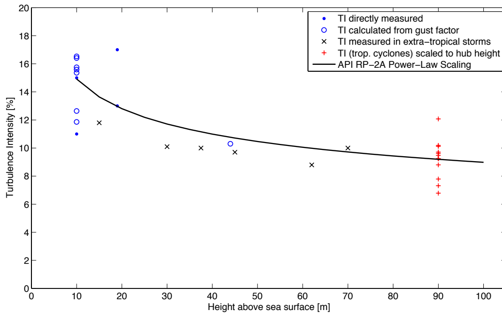
Figure A-8: Turbulence intensity (TI) in over-water tropical cyclones vs height. TI values from tropical cyclones are scaled to 90-meter height using a power-law relationship adapted from equation 2.3.2-3 in the API RP-2A-WSD standard. TI values measured in extra-tropical storms in the North Sea are also shown for comparison.
