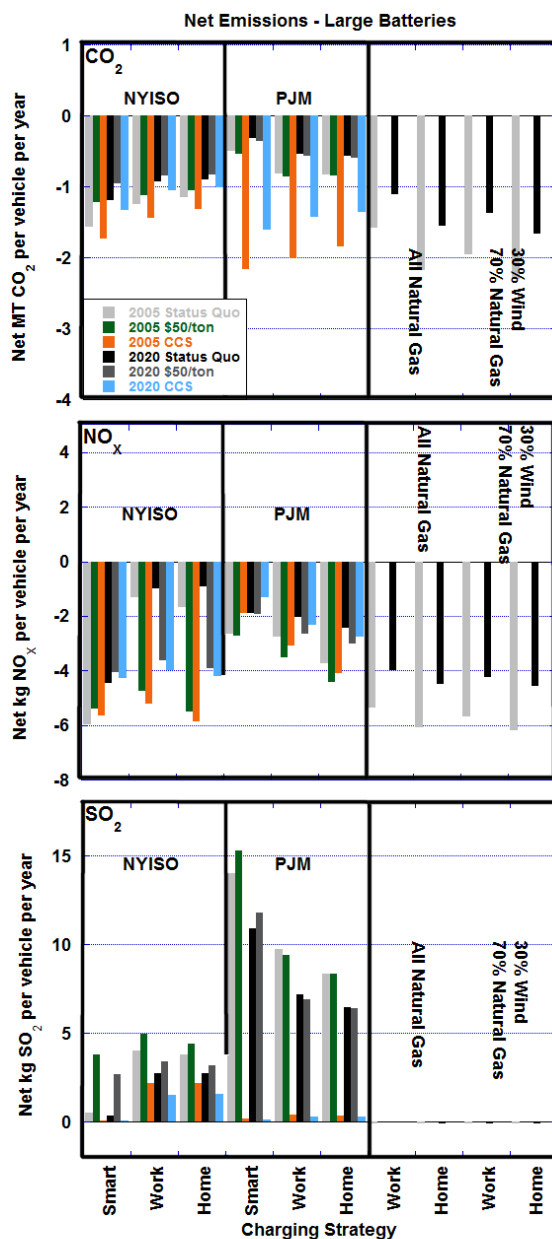
Figure 4S.19: Net emissions given 10% PHEVs and large batteries. Net metric tons of CO 2 , and net kg of NO x and SO 2 emitted per vehicle-year given PJM and NYISO generation mix as well as all natural gas and 30% wind combined with natural gas. For comparison, the predicted annual emissions per conventional vehicle using 2005 (22 mpg) and 2020 (35 mpg) efficiencies are 4.1 and 2.6 MT CO 2 , 10 and 6.4 kg NO x , and 0.20 and 0.13 kg SO 2 . Emissions for 2005 fleet and 2020 fleet are compared given the status quo (no carbon price) as well as a $50/ton CO 2 price and a $50/tonne CO 2 price in conjunction with CCS installed on coal plants. Different charging strategies are modeled to determine the timing of PHEV charging. 2005 generation mix assumed.
