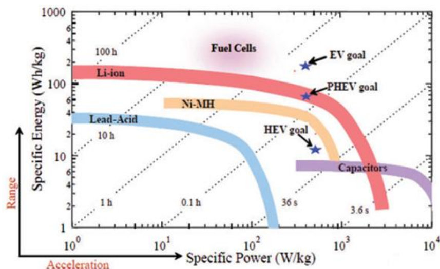
Figure 1.6 – Ragone plot comparing energy and power density of various battery types (adapted from [40])
