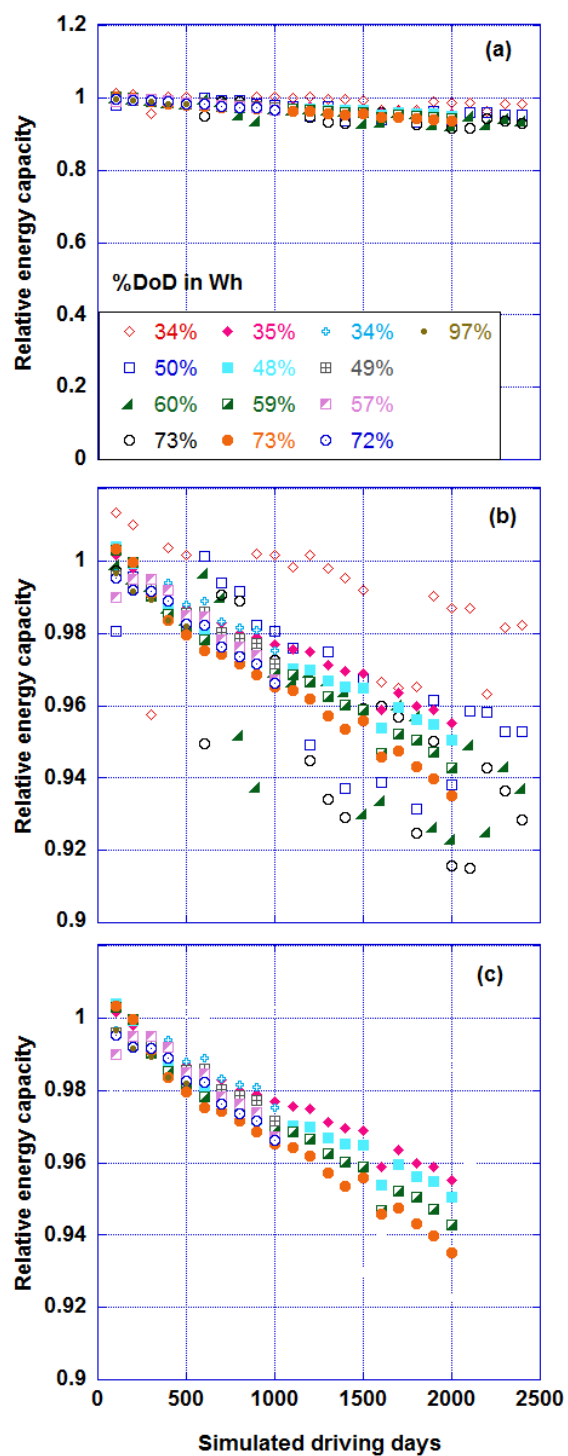
Figure 2.6 Degradation of cells versus driving days simulated (a) full range, (b) same information zoomed, (c) with highly variable cells from lot 1 dropped.
