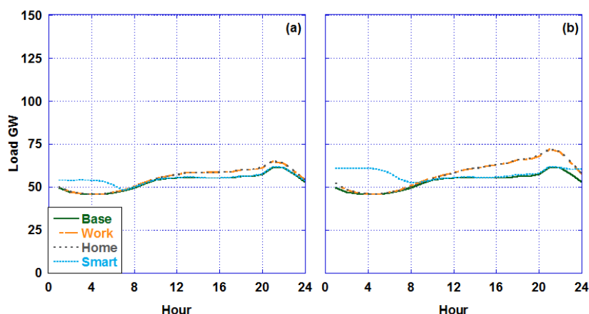
Figure 4S.1: Load on day of minimum hourly demand(Sunday, April 10, 2005) in PJM, 50% PHEVs with (a) small batteries and (b) large batteries
