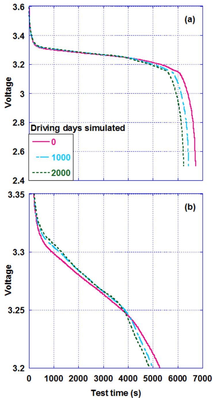
Figure 2.8 Voltage discharge profiles of a cell that reached an ultimate DoD value of 73% each driving day. The initial, 1000 th and 2000 th baseline discharge curves are shown.
