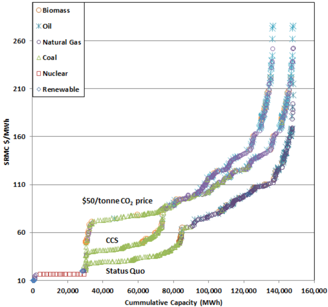
Figure 4S.7: SRMC curve for PJM based on yearly averages. Three different curves are shown for the three different carbon scenarios. Adding CCS decreased the SRMC of coal plants compared to a $50/tonne CO 2 price, but also results in a decrease in overall system capacity.
