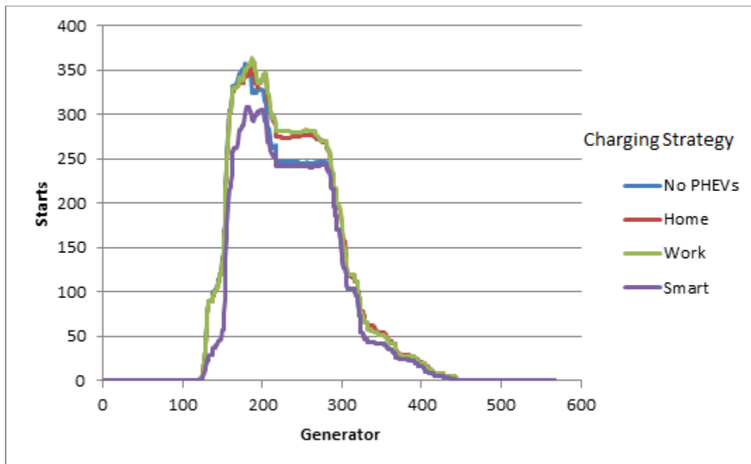
Figure 4S.9: Modeled plant starts in PJM given 10% PHEVs and large batteries
