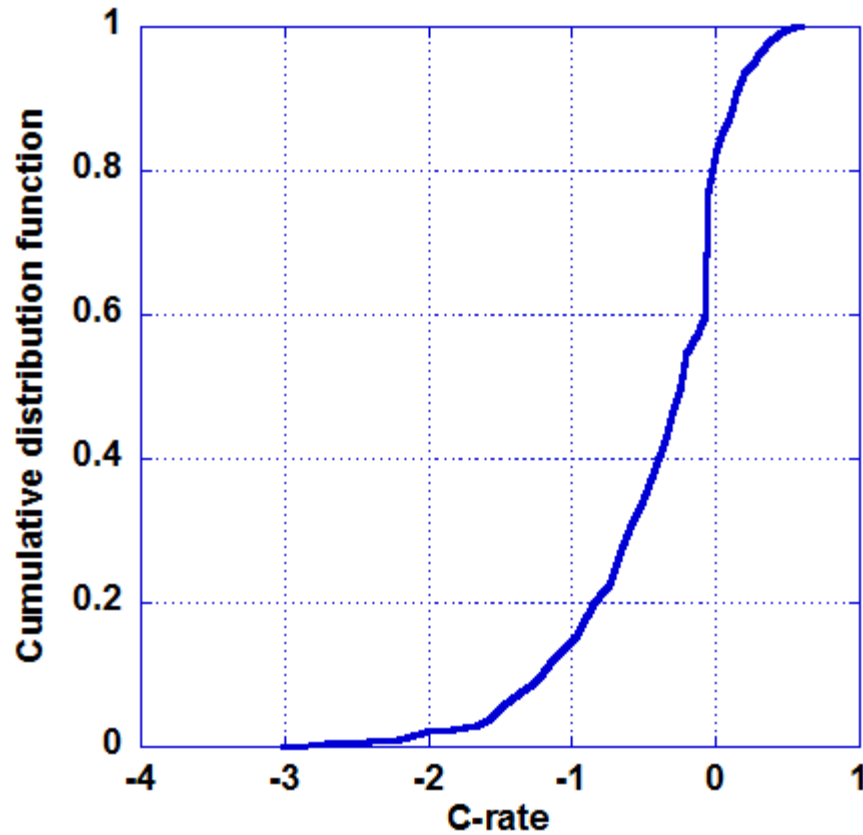
Figure 2.4 Cumulative distribution function of power requirements for daily driving (all 4 trips). Given large pack size the current rates are low most of the time. The near-vertical portion is a result of times when velocity and acceleration are low and the base load to run accessories dominates the power needs for vehicle.
