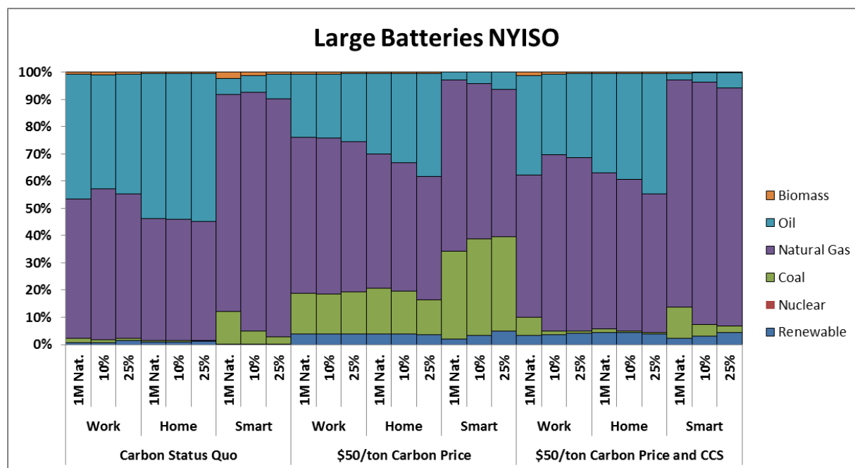
Figure 4S.13: Generation mix used to charge in NYISO given large batteries. Coal use for PHEVs predicted to increase given a carbon price. 2005 generation mix assumed.
