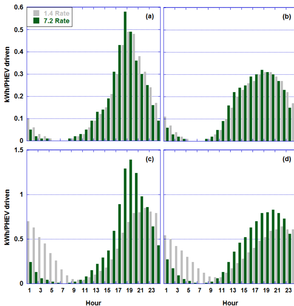
Figure 4S.5: A comparison of load given home charging with lower efficiency vehicles and two separate charge rates for (a) small batteries on a weekday, (b) small batteries on a weekend, (c) large batteries on a weekday, (d) large batteries on a weekend.
