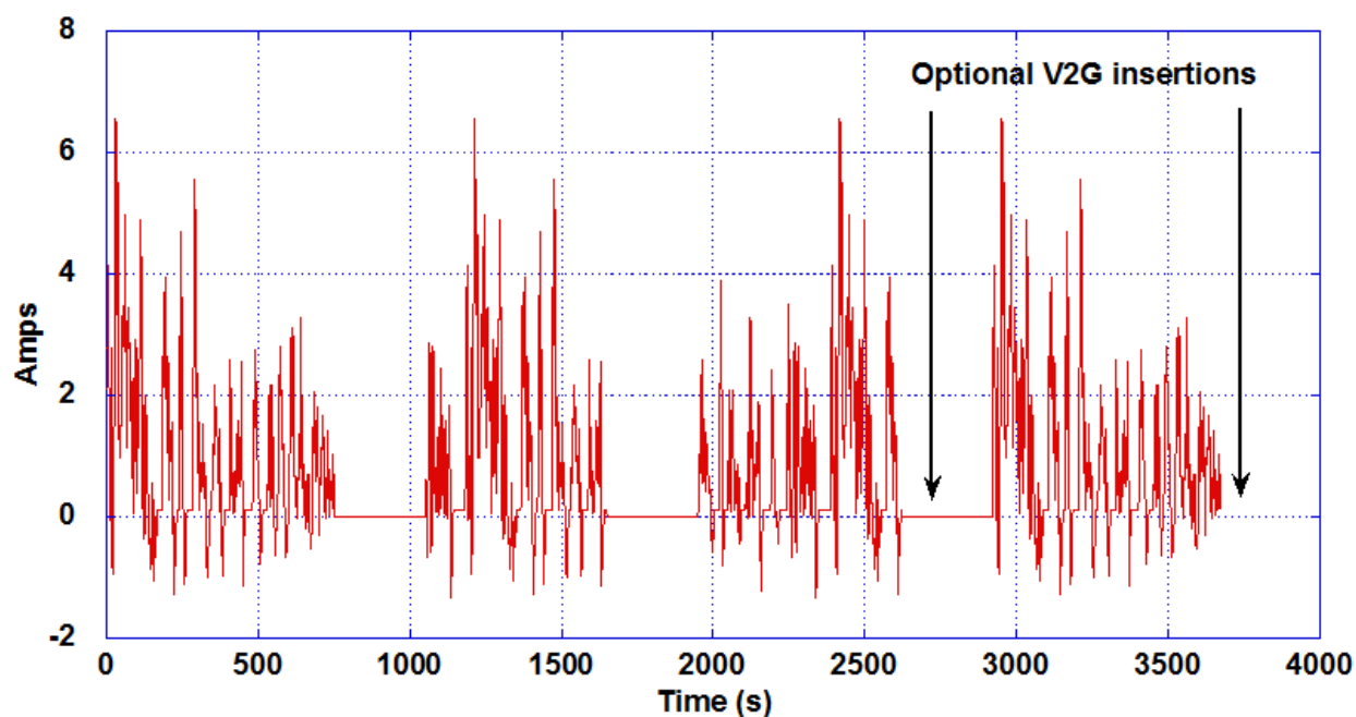
Figure 2.5 – Test current profile used to simulate driving day for cells showing all trips. The times after trips 3 and 4 when V2G discharge was simulated are indicated.
