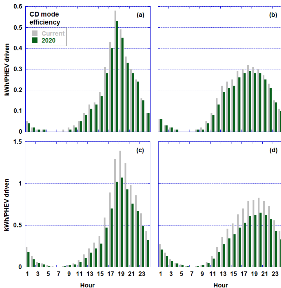
Figure 4S.3: Load per PHEV driven given home charging for (a) small batteries on a weekday, (b) small batteries on a weekend, (c) large batteries on a weekday, (d) large batteries on a weekend.
