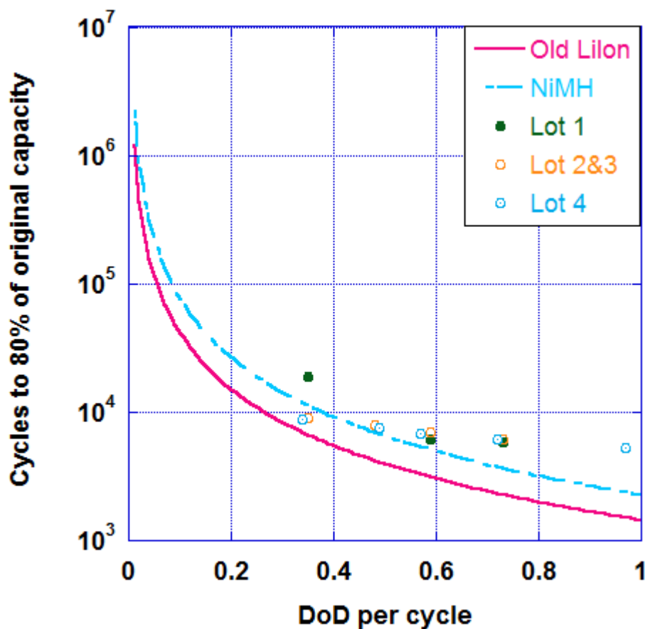
Figure 2.7 Laboratory results overlaid onto VARTA curves illustrating more linear response in cycle life as a function of depth of discharge for the cells tested.
