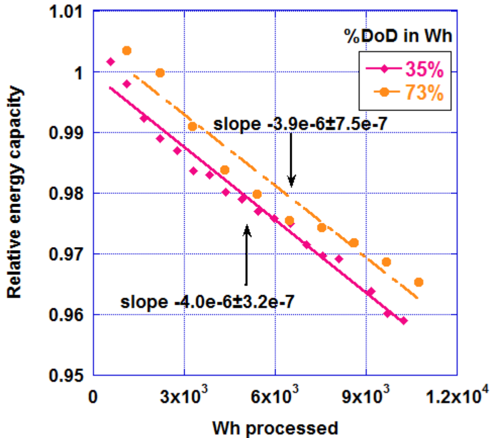
Figure 2.10 Capacity degradation as a function of energy processed for two cells tested with contrasting end-of-cycle depth of discharge values (35% and 73% DoD). The slight observed difference would indicate less degradation for higher DoD/cycle cell, however the 95% confidence interval of slopes overlaps for these fits, so they are not statistically discernible.
