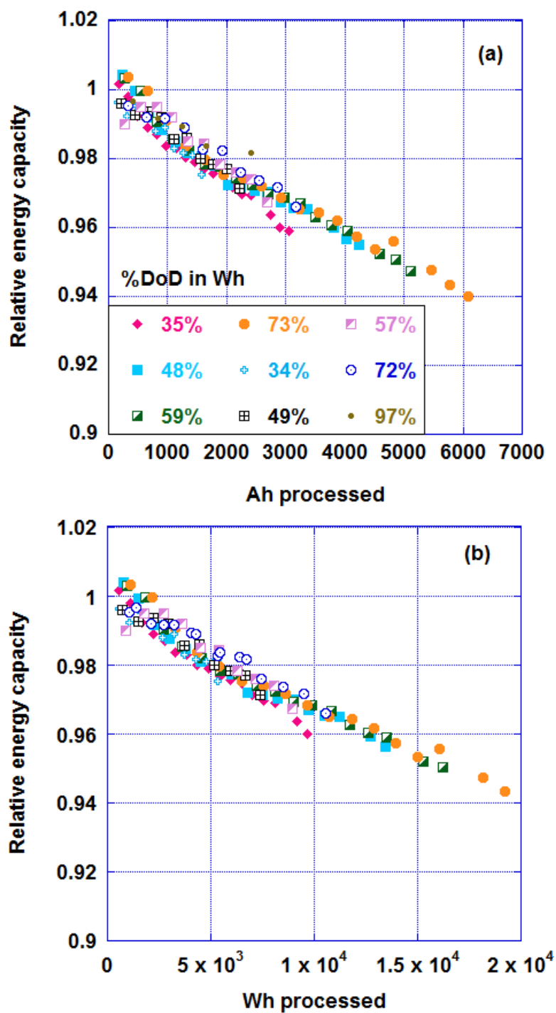
Figure 2.9 Degradation as a function of (a) capacity (Ah) processed by cell or (b) energy (Wh) processed by cell for all but lot 1 cells. Both appear linearly related, as expected given the nominally linear discharge profile of the LiFePO 4 /graphite system.
