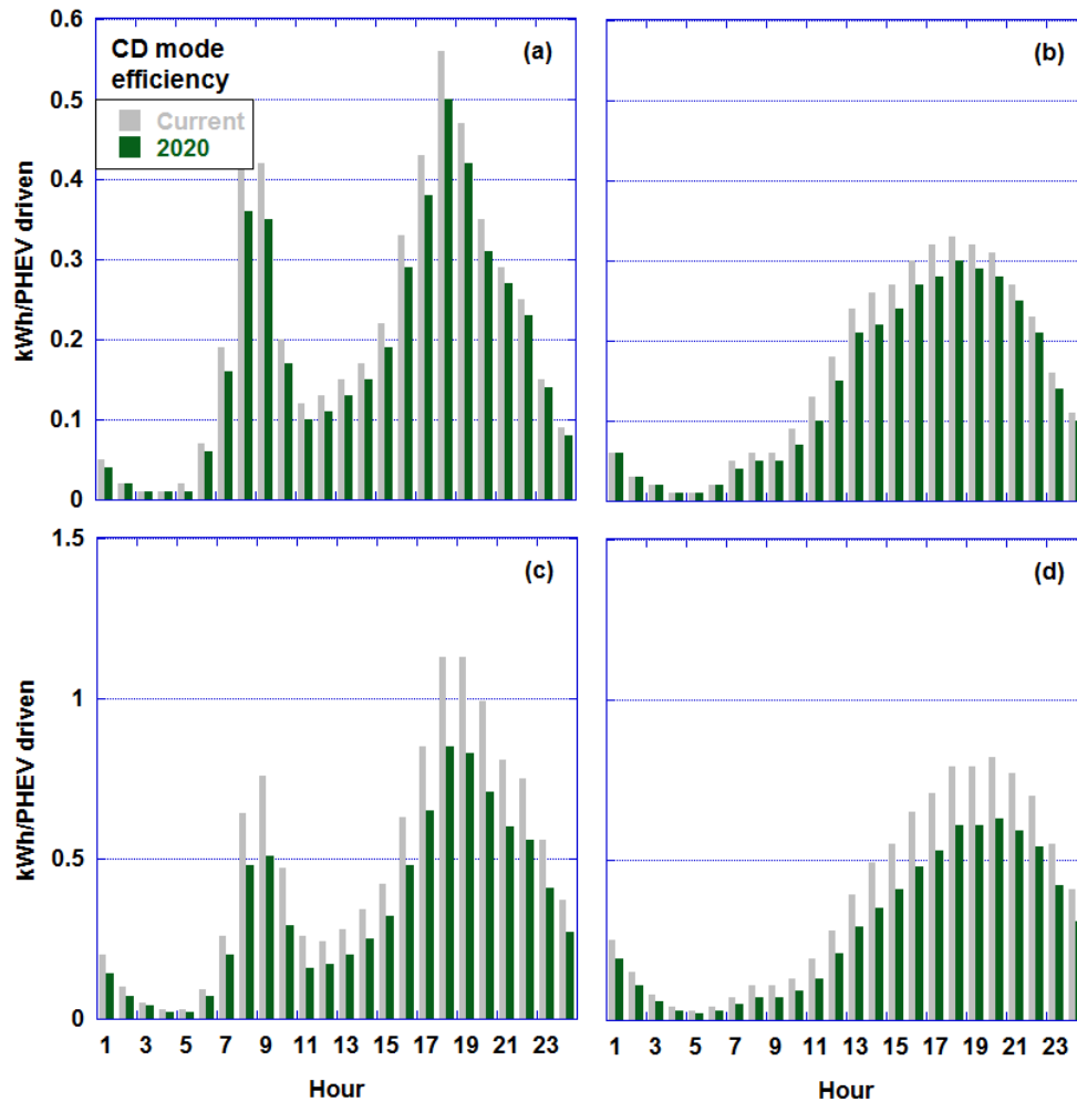
Figure 4S.4: Load per PHEV driven given work charging for (a) small batteries on a weekday, (b) small batteries on a weekend, (c) large batteries on a weekday, (d) large batteries on a weekend.
