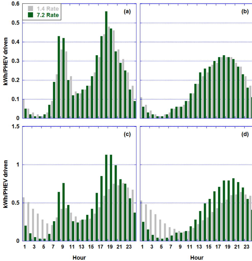
Figure 4S.6: A comparison of load given work charging with lower efficiency vehicles and two separate charge rates for (a) small batteries on a weekday, (b) small batteries on a weekend, (c) large batteries on a weekday, (d) large batteries on a weekend.
