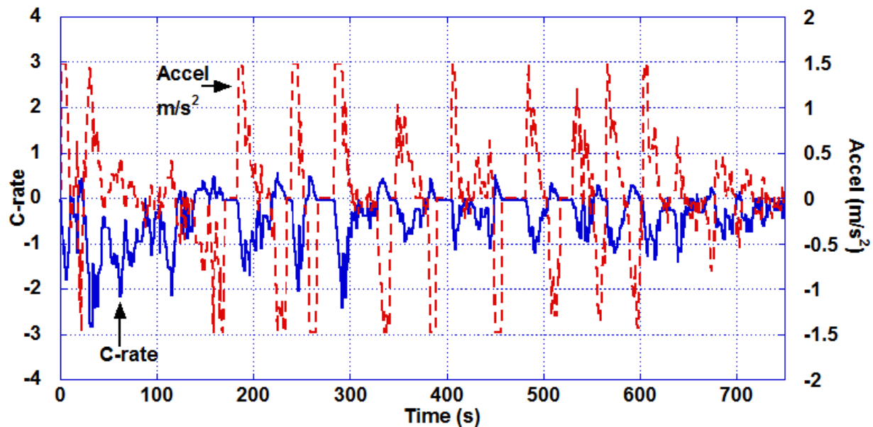
Figure 2.3 Example of relationship between acceleration and power required (in C-rate) for trips 1 and 4. A negative C-rate corresponds to discharge rate from pack. Deceleration can lead to regenerative braking if it is significant - in this case, around 7% of the energy is regained via regenerative braking.
