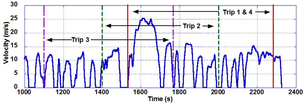
Figure 2.2 Portions of urban dynamometer driving schedule (UDDS) were chosen to closely match driving profile shown in Figure 2.1 in terms of duration and average velocity.
