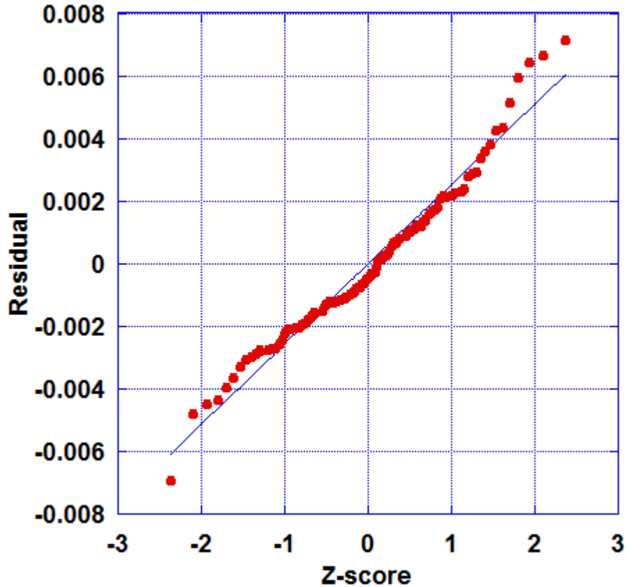
Figure 2.11 Q-Q plot shows errors are normally distributed for multiple linear regression. The line represents expected values for a normal distribution.
