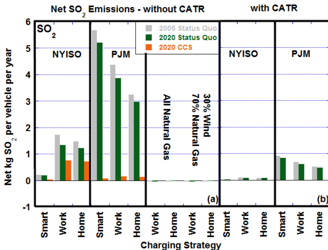
Figure 4.2: Net kg SO 2 emitted per vehicle-year given (a) PJM and NYISO generation mix of 2005, as well as all natural gas and 30% wind / 70% natural gas, and (b) PJM and NYISO with generator emissions factors for SO 2 reduced to comply with CATR. For comparison, the predicted annual emissions per conventional vehicle using 2005 (22 mpg) and 2020 (35 mpg) efficiencies are 0.20 and 0.13 kg SO 2 . Emissions for 2005 fleet and 2020 fleet are compared given the status quo (no CO 2 price) as well as a $50/tonne CO 2 price in conjunction with CCS installed on coal plants. Different charging strategies are modeled to determine the timing of PHEV charging. A similar figure for large batteries is included in the supporting information.
