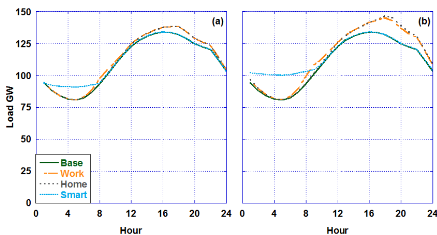
Figure 4S.2: Load on day of maximum hourly demand(Tuesday, July 26, 2005) in PJM, 50% PHEVs with (a) small batteries and (b) large batteries
