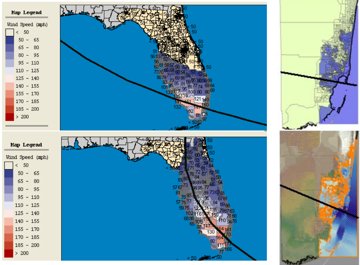
Figure 6.38. Wind speed (left) and storm surge (right) extents over the entire area for the “typical storm” for return periods of 500 years (top) and 1000 years (bottom) with respect to the location of Region 1.
