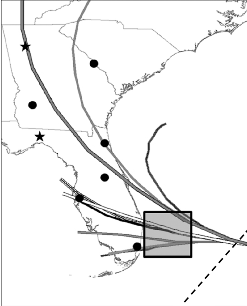
Figure 5.11. Visualization of the “Andrew-like” TCs examined in the study. Priors from Table 5.3-Table 5.5 are applied at the first point west of the dotted line. Nine different tracks are shown. Colors indicate eye bearing trajectory, (dark grey=clockwise change in eye bearing, white=no change in eye bearing, light grey=counter-clockwise change in eye bearing), and line types indicate eye translational speed (two black lines=high translational speed, solid color=medium translational speed, three black lines=low translational speed). Wind speed priors (not shown) are applied when the storm passes the dotted line, while wind-wave pump modifications are applied in the box.
