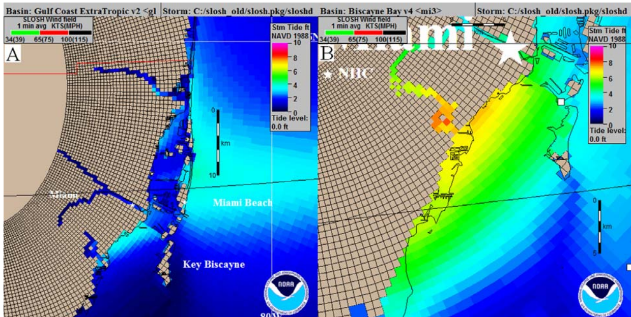
Figure 5.18. SLOSH output for two Andrew-like hurricanes with a direct hit on Miami. Figure A is the most intense storm making landfall closest to Miami (wind speeds increase by more than 5%, translational speed changes by less than 5%). Figure B is the most likely TC with a counter-clockwise change in eye bearing (wind speeds change less than 5%, translational speed decreases by more than 5%).
