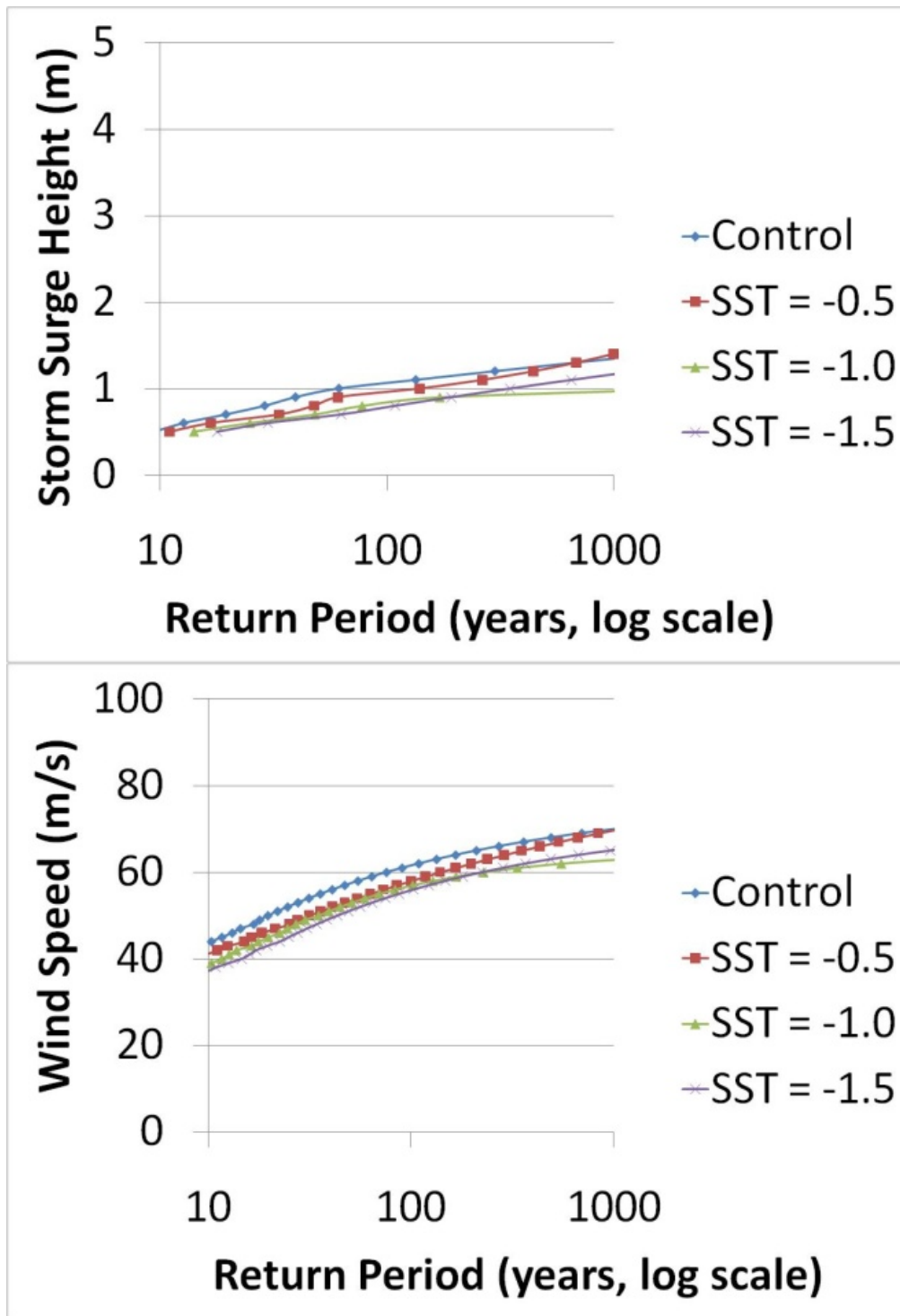
Figure 6.22. Storm surge (top) and wind (bottom) return level curves for Region 1.
