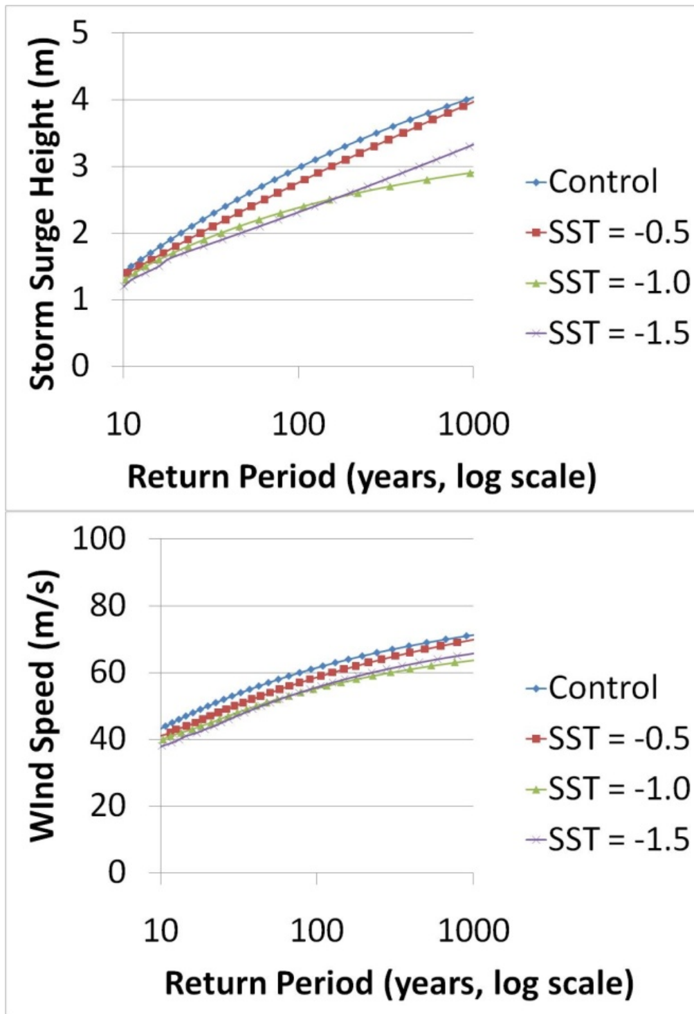
Figure 6.26. Storm surge (top) and wind (bottom) return level curves for Region 5.
