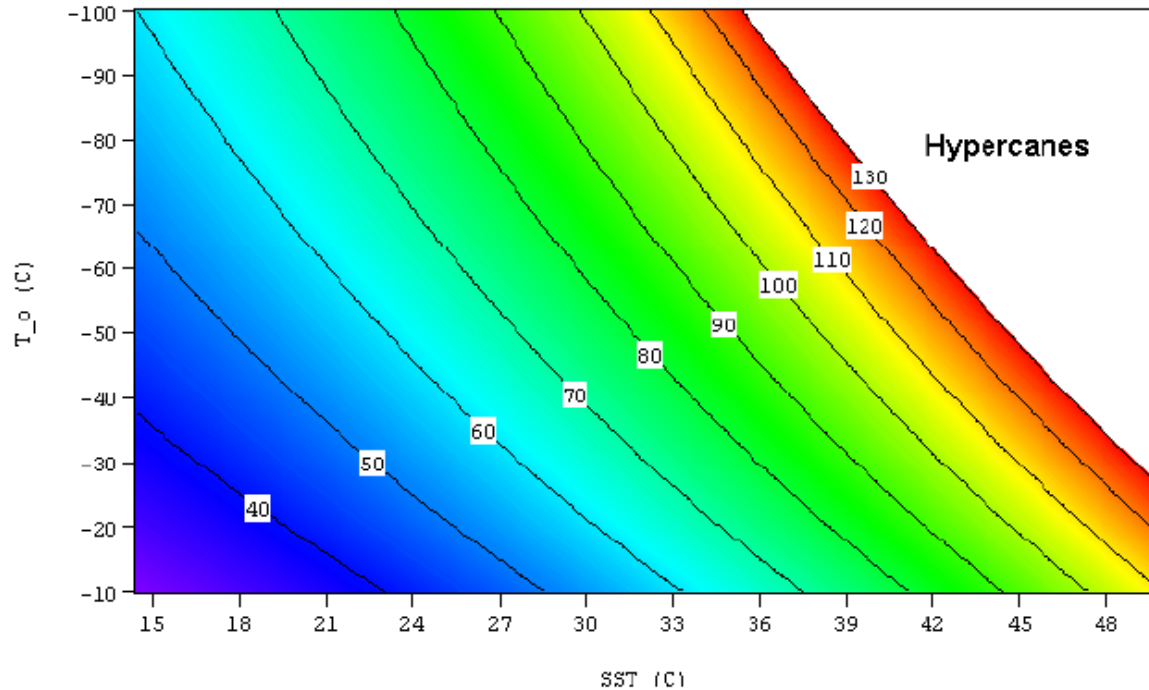
Figure 1.1. Contour plot of maximum wind speed (m/s, recall 1m/s=2.23mph) for sea surface temperature (SST) and storm top temperature ( T_o ). Enthalpy H=0.75 , C_K/C_D=1.2 . Figure courtesy of Emanuel, (7).
