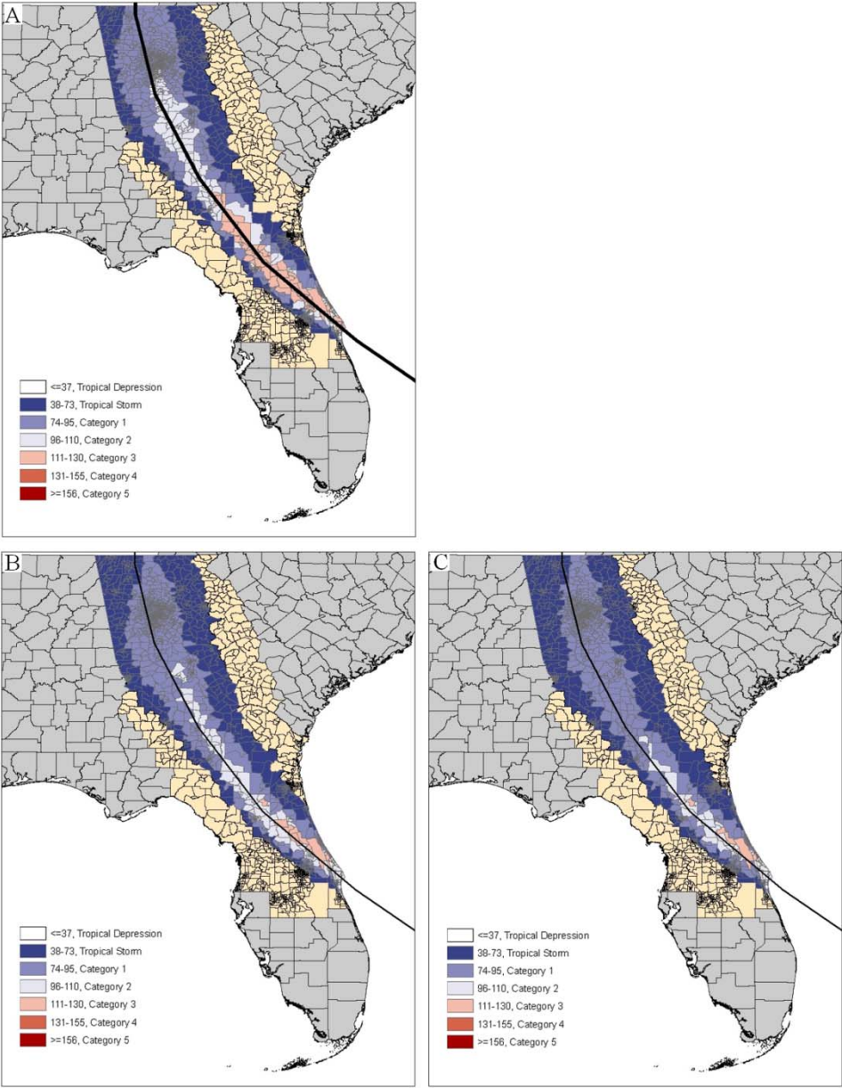
Figure 5.12. Maximum 1-minute sustained wind speed (knots) for the most likely scenario. Figure A is the most probable control scenario, with a wind speed change of 0%. Figure B is the control scenario with a wind-wave pump modification resulting in a 1°C decrease in SST. Figure C is the natural variability; the same eye translational speed and eye bearing, but decreased wind speed prior (~10%).
