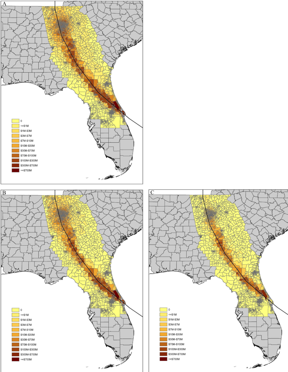
Figure 5.13. Total direct economic losses (log USD 2002) for the most likely technique. A: the most probable control trial (no wind speed change). B: Difference between control trial and the same trial with a 1°C SST decrease. C: Difference between control trial and the same trial with shuttering of all Florida and Georgia homes.
