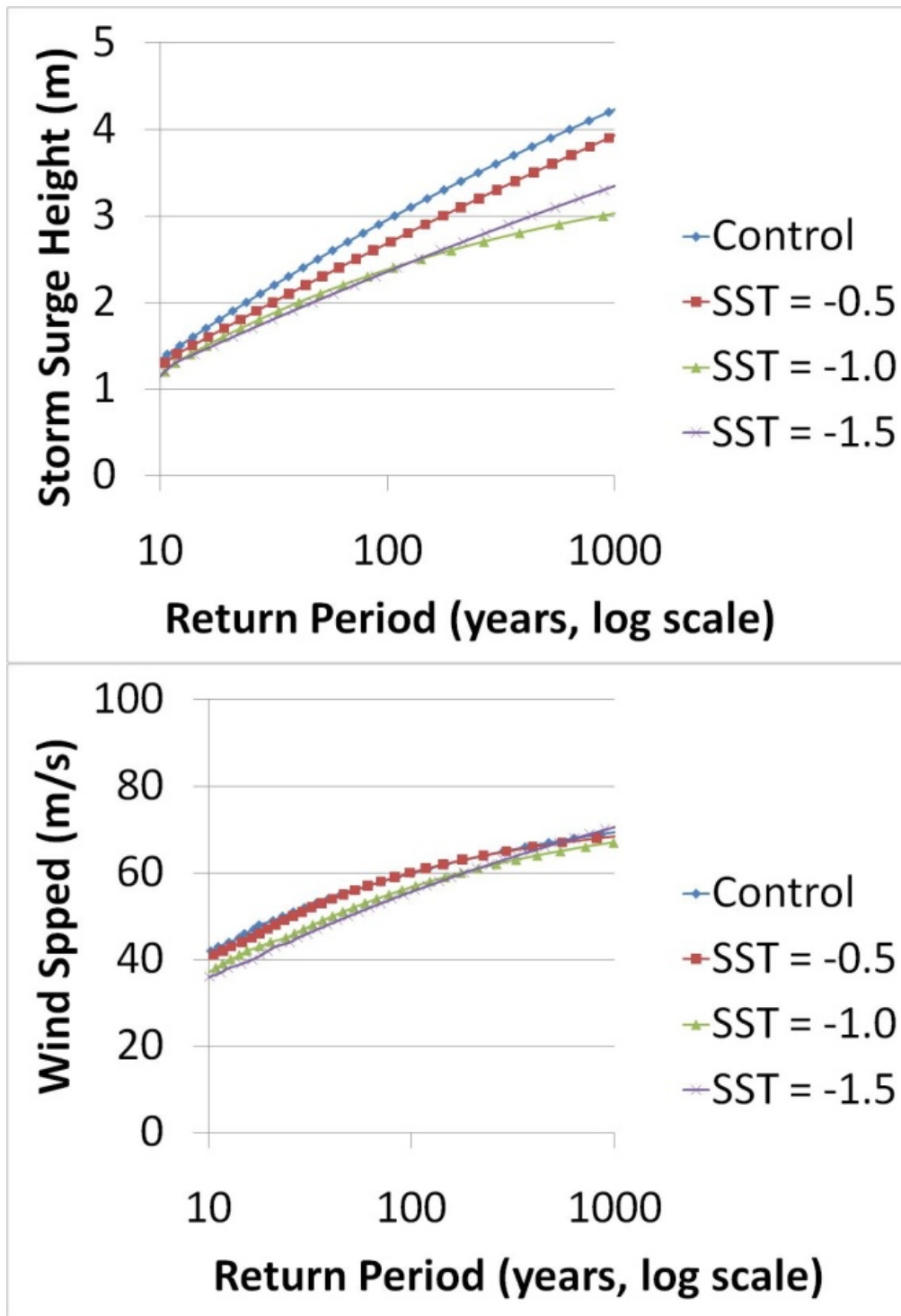
Figure 6.25. Storm surge (top) and wind (bottom) return level curves for Region 4.
