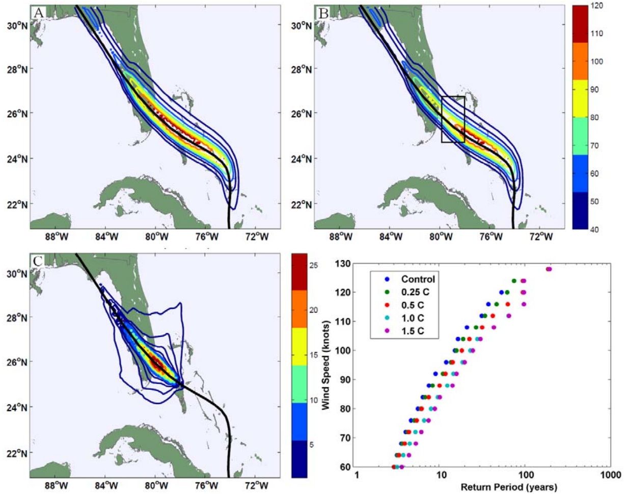
Figure 3.2. Results for the 500 hurricane track event set through the area east of Florida. Figure A is the maximum wind speed (knots) of a sample 100-year hurricane (contour bar to far right). Figure B is the maximum wind speed (knots) of a sample 100-year hurricane with a uniform SST decrease of 1°C in the box (25-27°N, 78-80°W). Figure C is the difference between Figure A and Figure B. Figure D is the maximum 1 minute sustained wind speed at 10m height as a function of return period and uniform SST decrease in the box (25-27°N, 78-80°W). Figures constructed by Kerry Emanuel.
