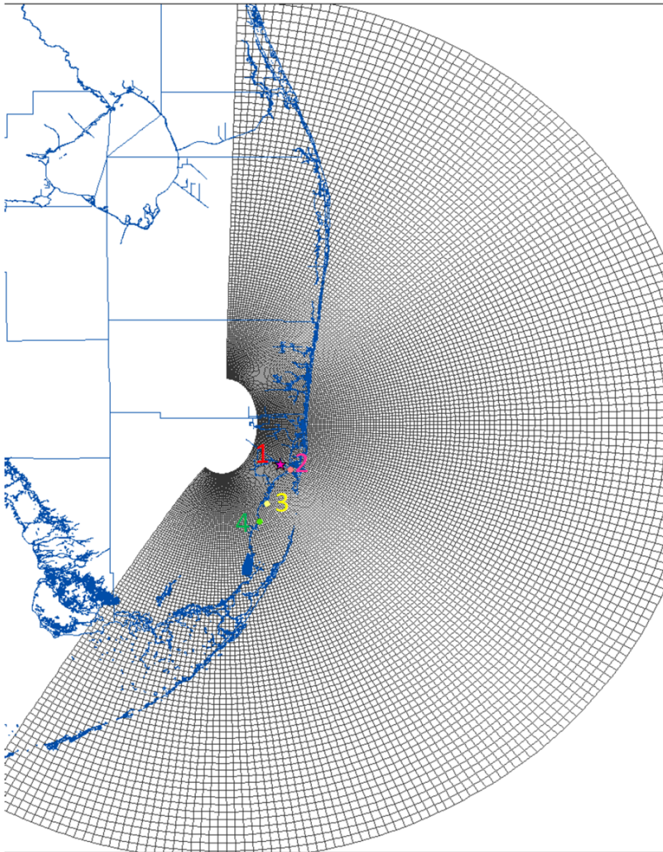
Figure 5.16. SLOSH hmi3 mesh and points of interest, courtesy of Ning Lin. Point 1 is Miami. Point 2 is a coastal point near to Miami. However, due to coastal bathymetry, both of these points are thought to have computationally intensive storm surge estimates, and thus storm surges here are less reliable. Point 3 and Point 4 are located in a less computationally intensive area, and are also chosen to be on the mesh grid (no interpolation between points). Point 3 is thought to have the best results.
