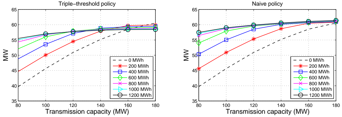
Figure 2.11 Wind energy sold per hour for different storage energy capacity levels under the triple-threshold policy (left) and the naive policy (right)
