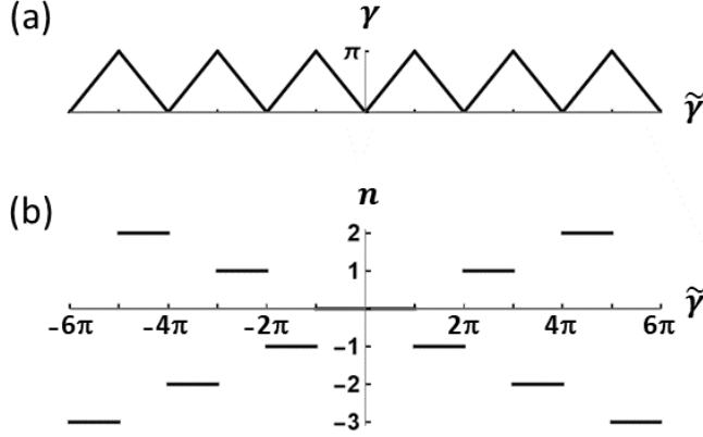
FIG 3. (a) Angular difference \gamma between initial and final locations for geodesic travel around a sphere, as a function of the total angular displacement \tilde{\gamma} . (b) Resulting values of winding number n .
