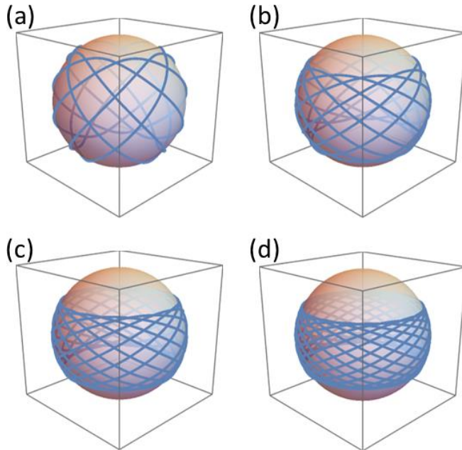
FIG 13. Qualitative, semiclassical paths associated with the azimuthally decomposed propagator. The \theta(t) part of the paths is in accordance with Eq. (77), associated with the Pösch-Teller potential, whereas the \phi(t) part is assumed to be given by Eq. (79). Results are for |m| = \ell = 1, 2, 3 , and 4 in (a) – (d) and are plotted using 7, 11, 15, and 19 periods, respectively, in the \theta(t) part of the motion.
