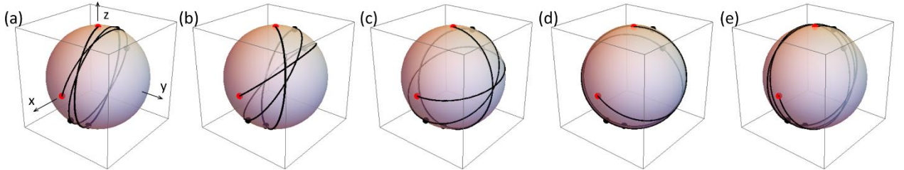
FIG 10. Similar caption as for Fig. 9, but with the paths here corresponding to winding numbers of 2 for (a) – (c) and -3 for (d) and (e). Total path lengths are approximately 4.519\pi , 4.667\pi , 4.938\pi , 5.253\pi , and 5.470\pi , respectively.
