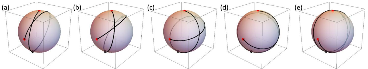
FIG 9. Paths composed of segments of circles extending between the same initial and final locations on a unit sphere as in Fig. 4, corresponding here to winding numbers of 1 for (a) – (c) and -2 for (d) and (e). The paths have take-off angles of \beta = 0.1\pi, 0.3\pi, 0.5\pi, 0.7\pi, and 0.9\pi , for (a) – (e), respectively, and their total lengths are approximately 2.515\pi, 2.642\pi, 2.898\pi, 3.225\pi, and 3.465\pi .
