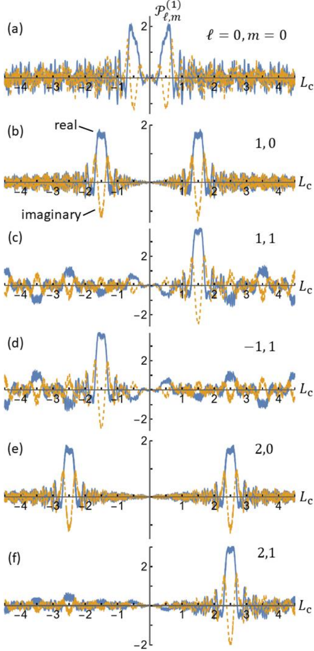
FIG 6. Path distributions \mathcal{P}_{\ell,m}^{(1)}(L_c, T) as given by Eq. (32), for integer values of \ell and m , as a function of the scalar characteristic angular momentum L_c that is determined by endpoints of a path. Real and imaginary parts of the distributions are shown by solid and dotted lines, as indicated. In all cases, peaks are obtained at one or both of the L_c values equal to \pm \hbar(\ell + 1/2) . Computations are performed for a travel time of T = 32\pi I/\hbar (units of \hbar = I = 1 are used in the plots).
