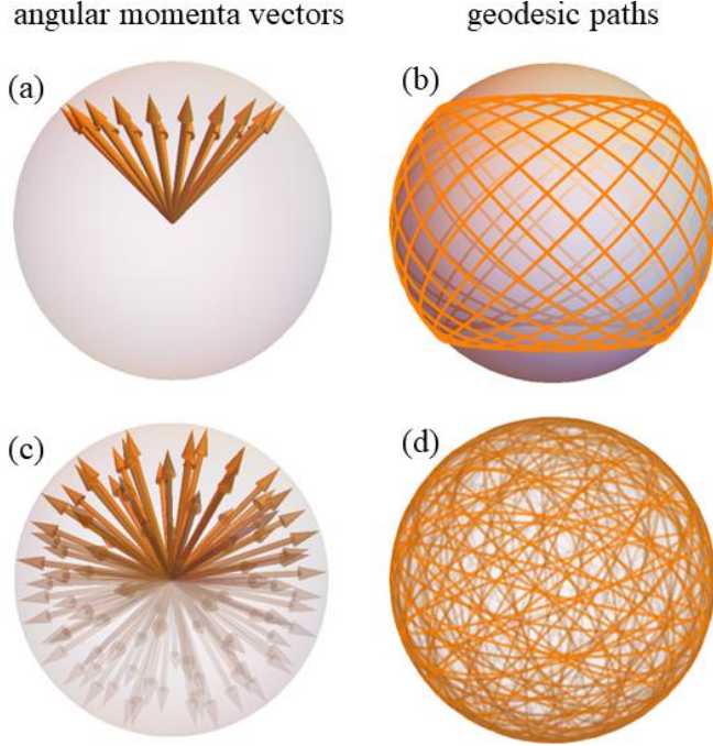
FIG 1. Comparison of distributions of geodesic (great circle) orbits for describing an eigenstates with \ell = 1 and m = 1 : (a) conventional result from the vector model, showing a distribution of vectors \mathbf{L}_c all with polar angle of \theta = \pi/4 ; (b) position-space orbits corresponding to the set of \mathbf{L}_c vectors shown in (a); (c) set of \mathbf{L}_c vectors as determined by the path distribution derived in the present work; (d) position-space orbits corresponding to the set of \mathbf{L}_c vectors shown in (c).
