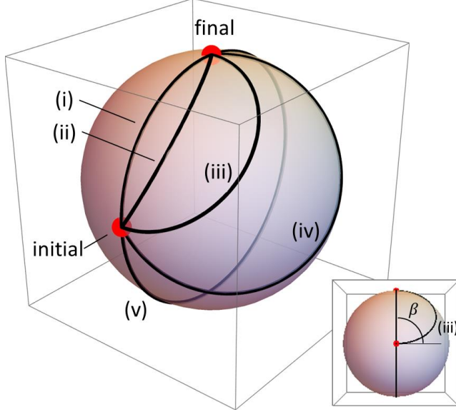
FIG 4. Circular paths extending between initial and final locations on a unit sphere, corresponding to winding numbers of 0 and -1 . Paths (i) and (v) are segments of a great circle, with angular lengths of \pi/2 and 3\pi/2 , respectively. Paths (ii) – (iv) are segments of small circles, with specified take-off angle \beta from the initial location (as shown in the inset for path (iii)) being \pi/4 , \pi/2 , and 3\pi/4 , respectively. The angular length of path (iii) is \pi , whereas for (ii) and (iv) it is approximately 0.608\pi and 1.392\pi , respectively.
