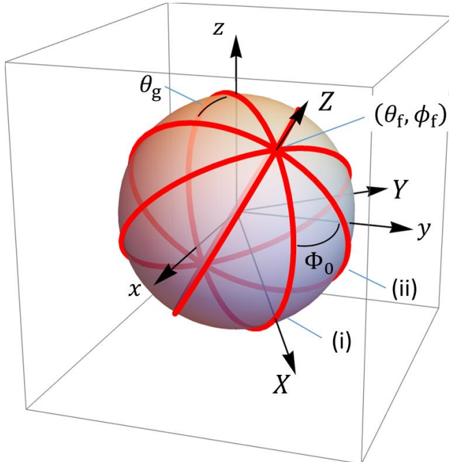
FIG 5. Great circles arrayed about a final location of a particle at (\theta_f, \phi_f) . A rotated coordinate frame (X, Y, Z) is indicated, aligned to the great circles, with (\Theta_f, \Phi_f) = (0, 0) in the rotated frame. Two great circles are indicated by (i) and (ii). The angle between them is labeled \Phi_0 , whereas the angle between the plane containing great-circle (ii) and the z -axis is labeled \theta_g .
