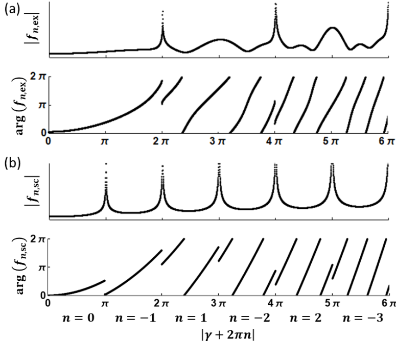
FIG 2. Comparison of (a) the exact propagator, and (b) the semiclassical propagator, for free-particle motion in S^2 . Magnitude and phase (modulo 2\pi ) of each propagator is shown, plotted as a function of |\gamma + 2\pi n| where \gamma is the angle subtended between initial and final locations ( 0 \leq \gamma \leq \pi ) and n is the winding number. The travel time is taken to be T = 3 , using units of \hbar = I = 1 .
