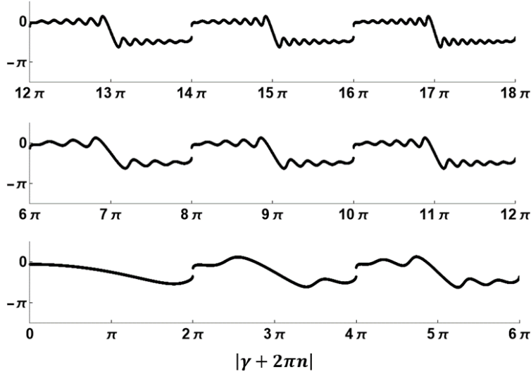
FIG 8. Phase difference between exact and semiclassical propagators, not including the discontinuous phase jumps of each. Results are for a travel time of T = 3 . The panels have differing ranges of |\gamma + 2\pi n| values, as indicated on the respective horizontal axes.
