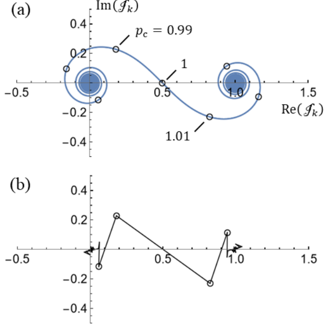
FIG 1. (a) Phasor diagram of \mathcal{F}_k(p_c, x_f, T) from Eq. (13), as a function of p_c varying between -\infty and +\infty , for an eigenstate with k = 1 at a travel time of T = 10^4 . The black circles indicate p_c values of 0.97, 0.98, 0.99, 1, 1.01, 1.02, and 1.03 (with the middle three values labeled). Units of \hbar = M = 1 are used. (b) Decomposition of the curve in (a) into line segments that join a set of p_c values spaced by 0.02.
