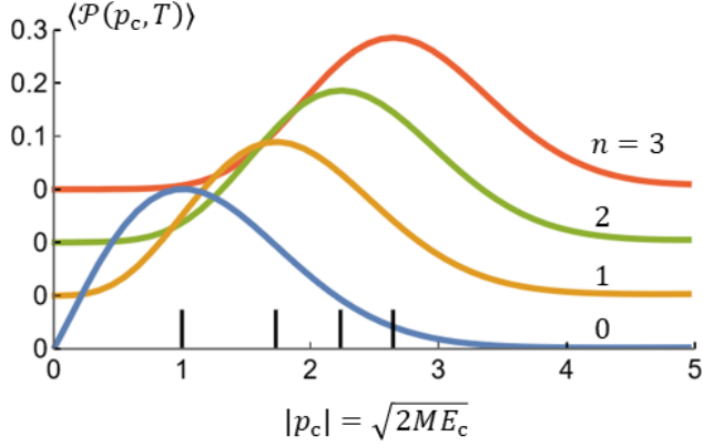
FIG 7. \langle \mathcal{P}_n(p_c, T) \rangle from Eq. (36), as a function of |p_c| , for the n = 0, 1, 2 , and 3 eigenstates of the harmonic oscillator, evaluated for a travel time of T = 32\pi (using units of \hbar = M = 1 and taking \omega = 1 ). The plots are vertically offset from one another, for clarity. The thick lines near the horizontal axis indicate |p_c| -values of 1, \sqrt{3} , \sqrt{5} , and \sqrt{7} , corresponding to \sqrt{2ME_n} for the various eigenstates.
