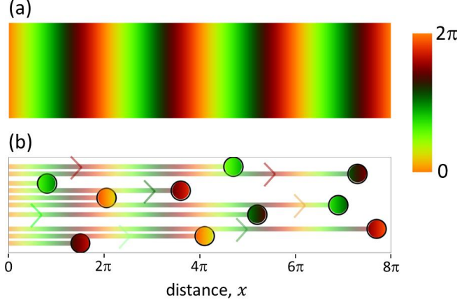
FIG 3. (a) Wave function for free-particle motion in \mathbb{R}^1 , with phase indicated by the color scale shown on the right-hand side. (b) Dominant paths for the motion. Final locations are indicated by circles, filled by a color indicating the phase. (The vertical extent of the plots has no physical meaning; it is used only to provide space to show the various paths).
