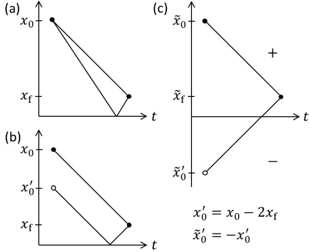
FIG 5. Space-time diagrams of paths for reflection from a hard wall, showing (a) space with x > 0 and paths with same initial location but different speeds, (b) space with x > 0 and paths with different initial locations but same speed, (c) space -\infty < \tilde{x} < \infty and paths as in (b), with different initial locations but same speed. Expressions for the initial locations x'_0 and \tilde{x}'_0 of cases (b) and (c) are listed below panel (c), applicable to large travel distance and x_0 \gg x_f .
