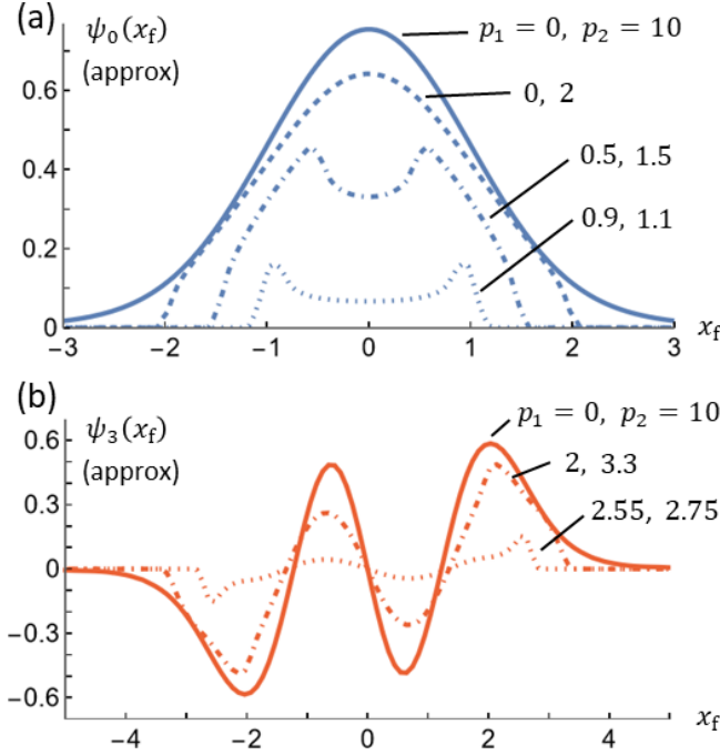
FIG 8. Approximations to the harmonic-oscillator wave function \psi_n(x_f) computed according to Eq. (39) using paths extending over |p_c| \in (p_1, p_2) for the p_1 and p_2 values indicated. Computations are for a travel time of T = 32\pi (using units of \hbar = M = 1 and taking \omega = 1 ). Results are shown for states with (a) n = 0 and (b) n = 3 (with \sqrt{2ME_n} = 1 for (a) and \sqrt{2ME_n} = \sqrt{7} \approx 2.65 for (b)).
