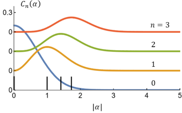
FIG 10. Overlap squared between a harmonic oscillator eigenstate and a coherent state |\alpha\rangle , for the n = 0, 1, 2 , and 3 eigenstates (using units of \hbar = M = 1 and taking \omega = 1 ). The plots are vertically offset from one another, for clarity. The thick lines near the horizontal axis indicate |\alpha| -values of 0, 1, \sqrt{2} , and \sqrt{3} , corresponding to expectation values for the energy of the coherent states that equal the energy eigenvalues of the respective eigenstates.
