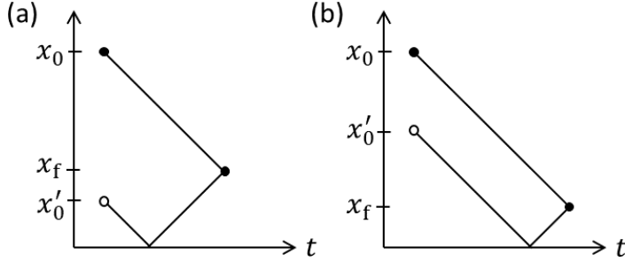
FIG 6. Space-time diagrams of paths for reflection from a hard wall, shown in a manner analogous to that of Fig. 5(b), but now showing two different travel times in (a) and (b).
