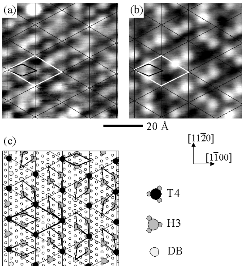
Figure 5 Simultaneously-acquired dual bias images of the 5 \times 5 reconstruction. Sample biases are +2.0 V and -2.0 V with gray scale ranges of 0.5 Å and 0.6 Å for (a) and (b), respectively. A 5 \times 5 grid is superimposed on each image with the corners located on the bright features seen in (a). Shown in (c) is the same 5 \times 5 grid where the underlying primitive lattice is shown in empty circles. Black circles are T4 adatom sites. Dark gray circles are H3 adatom sites. Light gray circles are DB (dangling bond) sites. The small diamond shapes represent the basic structural unit for the 5 \times 5, which is found in three possible orientations throughout the surface.
