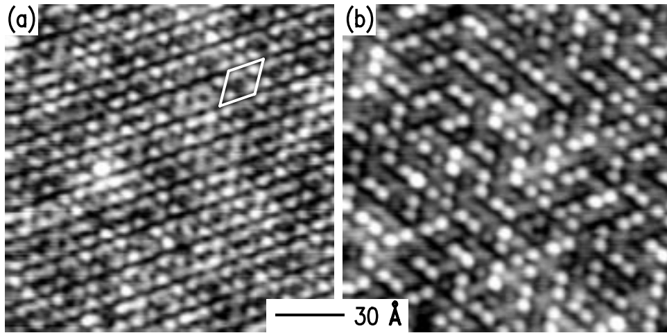
Figure 4 Simultaneously-acquired dual bias images of the 5×5 reconstruction. Sample biases are +1.0 V and -1.0 V with gray scale ranges of 0.5 Å and 0.9 Å for (a) and (b), respectively.
