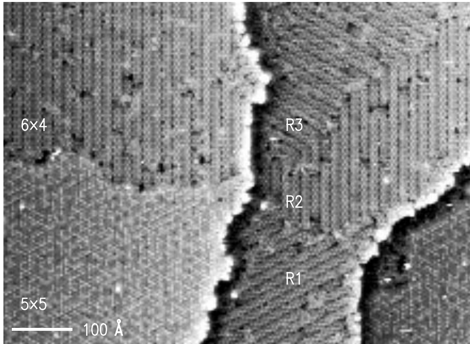
Figure 1 STM image of Ga-face showing 5×5 and 6×4 reconstructions. The three terraces are separated by single bilayer-height steps (1 bilayer = 2.59 Å). R1, R2, and R3 indicate three different rotational domains of the row-like 6×4 reconstruction. Sample bias = -1 V; tunnel current = 0.075 nA. The image is displayed with a local area background subtraction.
