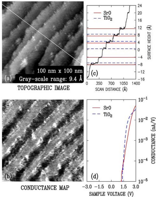
FIG. 2 (Color online) (a) Topographic image and (b) conductance map of the cleaved \text{SrTiO}_3(100) surface obtained with a sample bias of +3.0 \text{ V} . At this bias, bright conductance stripes occur for \text{SrO} termination while dark stripes occur for \text{TiO}_2 termination. (c) A height profile obtained along the specified path in (a). Red solid lines show \text{SrO} -terminated terraces while blue dashed lines show \text{TiO}_2 -terminated terraces. (d) Conductance versus voltage spectra averaged across their respective \text{SrO} - and \text{TiO}_2 -
