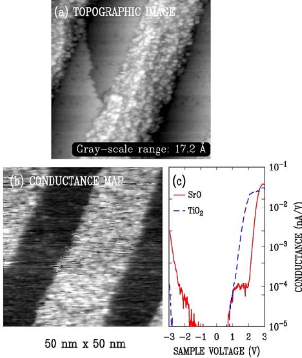
FIG. 3 (Color online) (a) Topographic image, and (b) conductance map of the cleaved \text{SrTiO}_3(100) surface obtained with a sample bias of +1.5 V. At this bias, bright conductance stripes occur for \text{TiO}_2 termination while dark stripes occur for SrO termination. (c) Conductance versus voltage spectra averaged across their respective SrO- and \text{TiO}_2 -terminated terraces. The Fermi level occurs at 0 V. Note: titanium coating was used on this sample.
