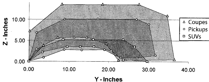
Fig. 29. The front fender curve local coordinate system. The grey area surrounded by a symbol shows the allowable range for the control points to stay within the designated vehicle class.
