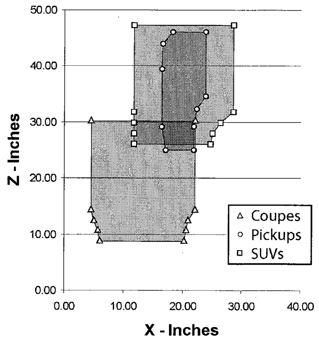
Fig. 38. The grill curve global coordinate system. The grey area surrounded by a symbol shows the allowable range for the control points to stay within the designated vehicle class.
