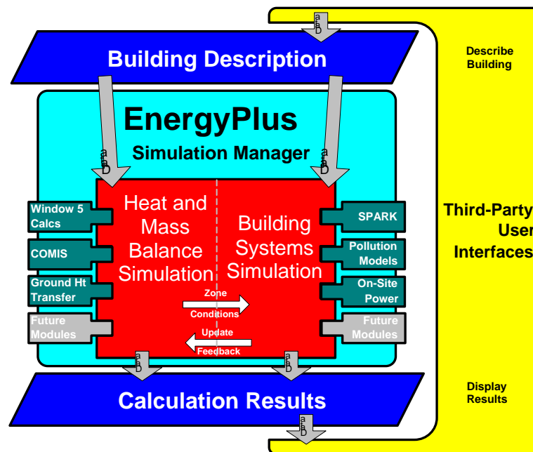
Figure 1. Overall Structure of EnergyPlus
