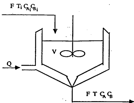
Figure 3. The nonisothermal CSTR.
