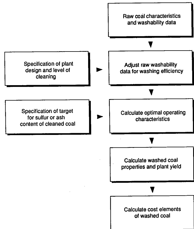
Figure 2. Schematic of model procedures.
