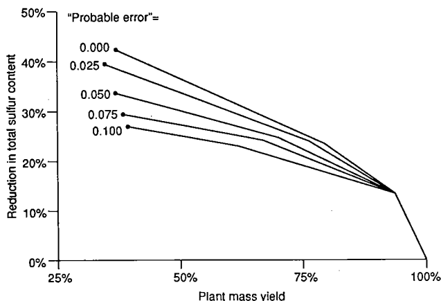
Figure 3. Effect of probable error in sulfur reduction for a typical Pennsylvania coal.
