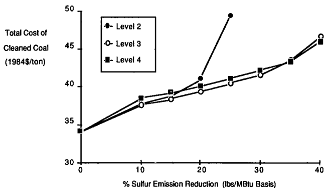
(a) 1.71%S Upper Freeport Coal
