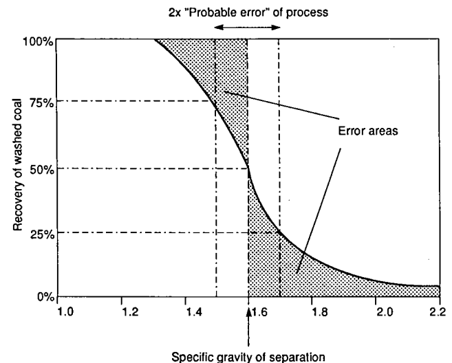
Figure 1. "Partition" curve for coal washing in a Baum jig.
