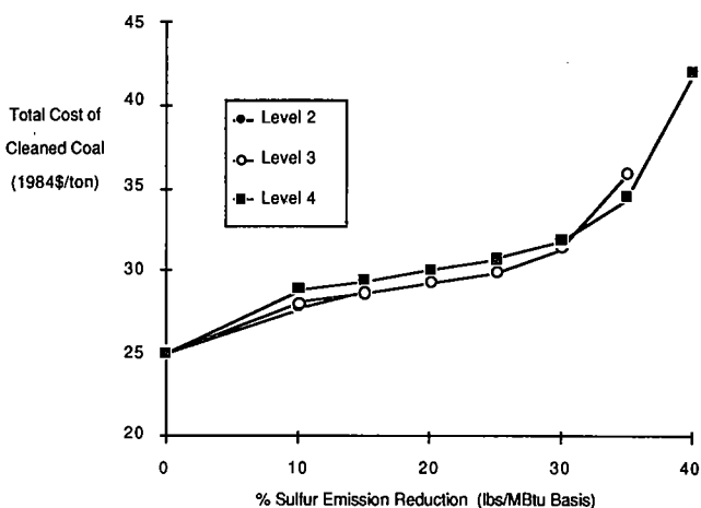
Figure 4. Predicted sulfur reduction costs for three U.S. coals.
