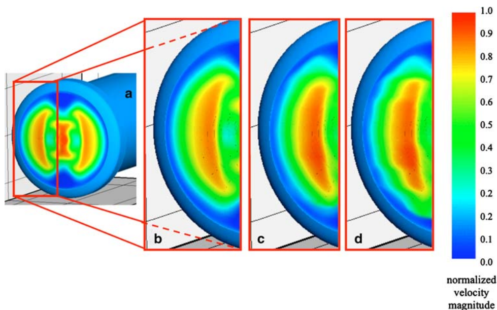
Fig. 6 Cutaway views of a jet downstream from the bileaflet valve. Velocity magnitudes within the light blue chamber have been normalized by the maximum value in each fluid domain. Shown are a the complete CFD solution, b the region of interest from CFD, and c and d that same region from the ACGI2 and cubic spline reconstructions, respectively
