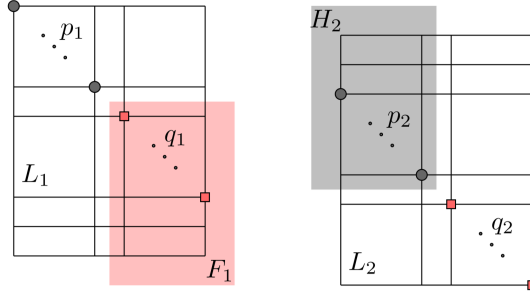
Figure 8.4: F_1 in G_1 and H_2 in G_2
