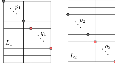
Figure 8.1: L_1 in G_1 and L_2 in G_2
