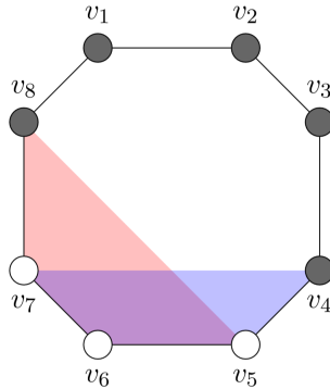
Figure 4.4: An example in \mathbb{R}^2
