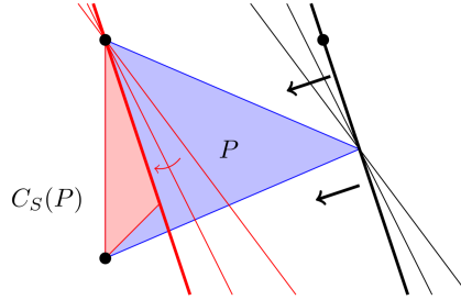
Figure 5.2: Some facets are not defined by S -CG inequalities
