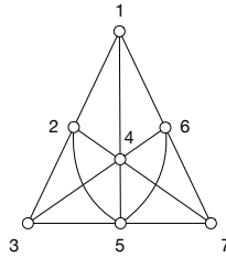
Figure 1.2: The Fano plane
