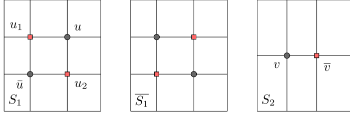
Figure 8.3: S_1 , \overline{S_1} , and S_2
