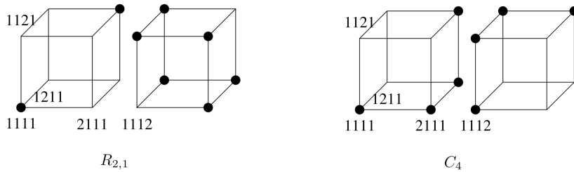
Figure 1.6: R_{2,1} and C_4
