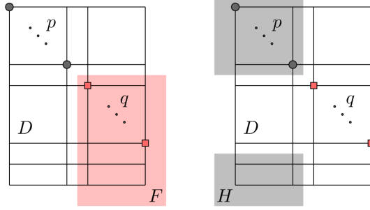
Figure 8.2: F and H in G_1
