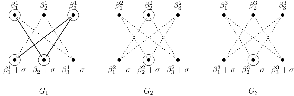
Figure 9.3: The subgraph of H_{n,\alpha} after deleting the vertices
