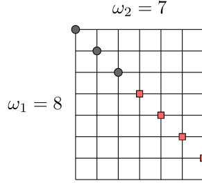
Figure 7.3: A general diagonal of H_{8,7}
