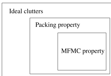
Figure 1.1: Classes of clutters
