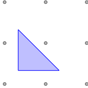
Figure 2.2: P_2 in \mathbb{R}^2
