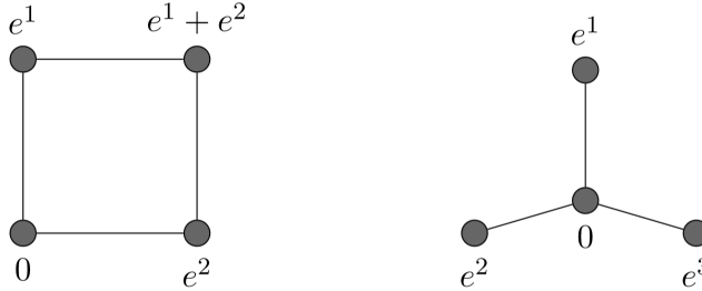
Figure 4.1: Square and star with \bar{x} = 0
