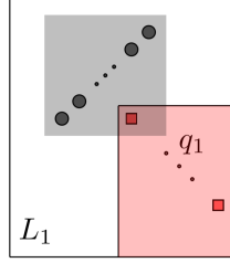
Figure 8.5: L_1 in G_1 : a contradiction
