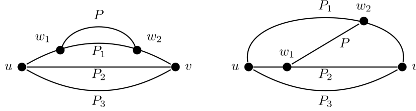
Figure 9.7: w_1, w_2 \notin \{u, v\}
