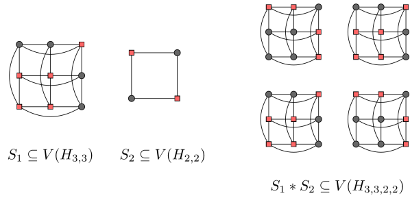
Figure 1.5: An example of taking the reflective product of two sets
