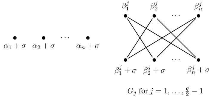
Figure 9.2: The edges of size 1&2 of H_{n,\alpha}
