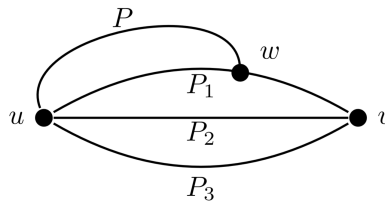
Figure 9.6: w \notin \{u, v\}
