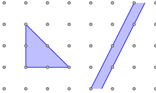
Figure 2.4: Thin simplicial cylinders in \mathbb{R}^2
