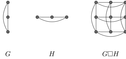
Figure 1.3: Cartesian product example
