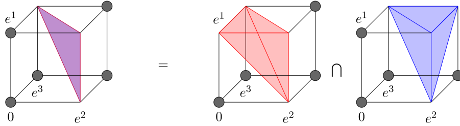
Figure 4.3: An example of decomposition around a cut vertex in \mathbb{R}^3
