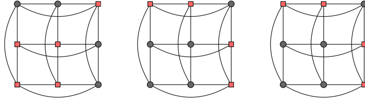
Figure 7.1: A set in V(H_{3,3,3}) that has R_{1,1} as a set-restriction
