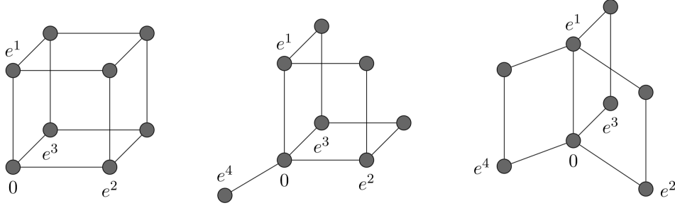
Figure 4.2: Cube, tulip, and propeller with \bar{x} = 0
