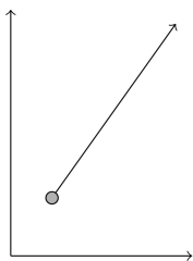
Figure 2.3: P in \mathbb{R}^2
