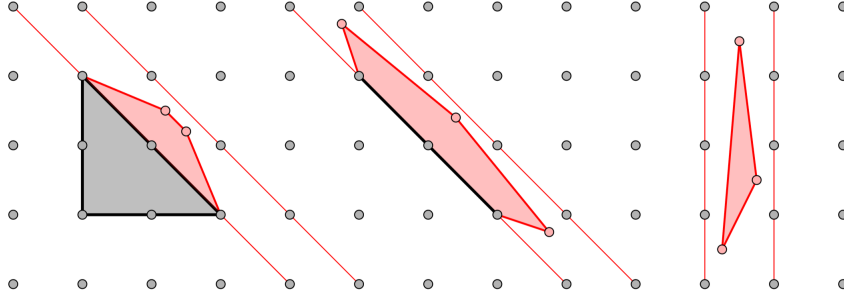
Figure 2.1: When one Chvátal-Gomory inequality is sufficient in \mathbb{R}^2
