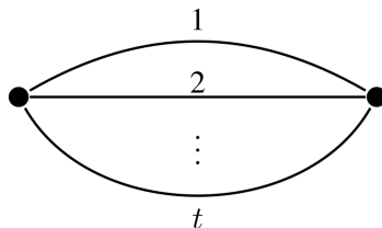
Figure 9.1: Graph on two vertices and parallel edges
