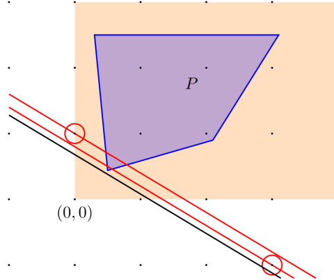
Figure 5.1: Illustration of an S -CG inequality
