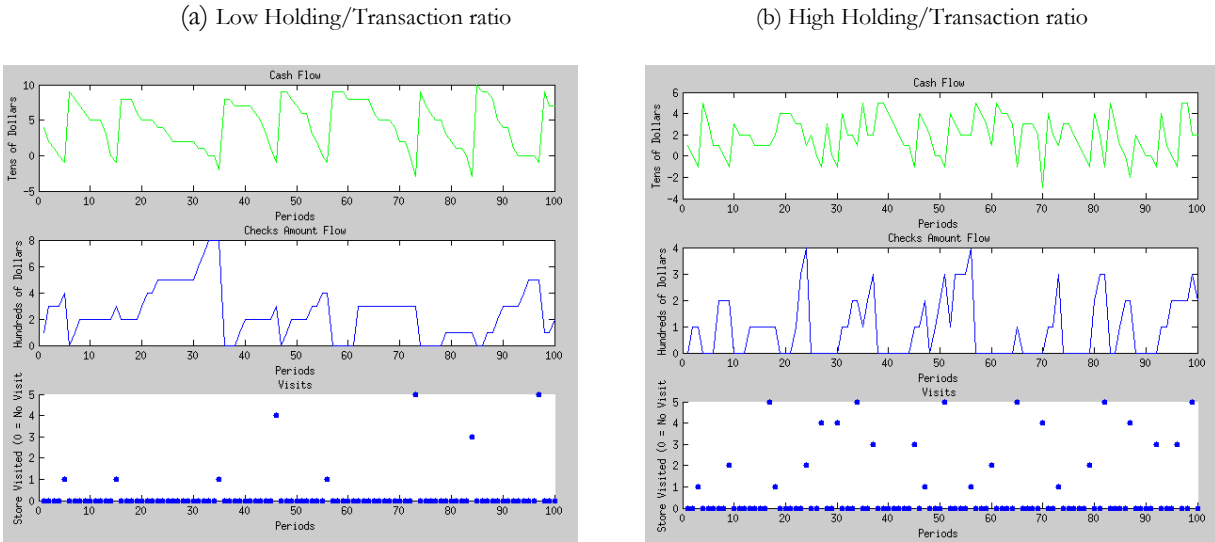
Figure 5. Model workings, bank activities vs periods.
