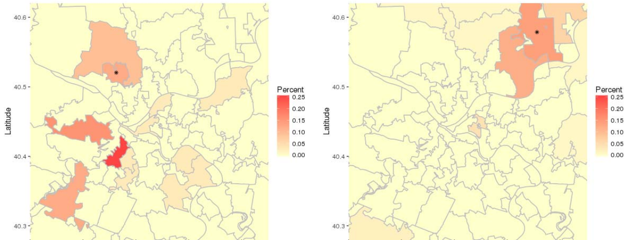
Figure 3. Two examples of consumer observed activity during 6 months
