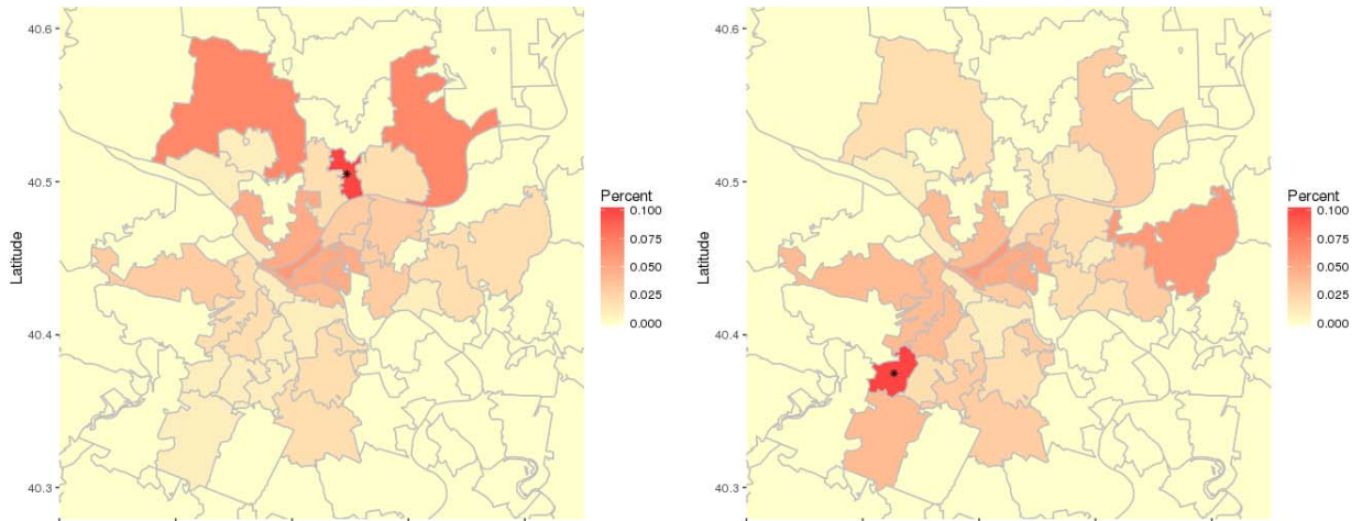
Figure 4. Two examples of connectivity regions.
