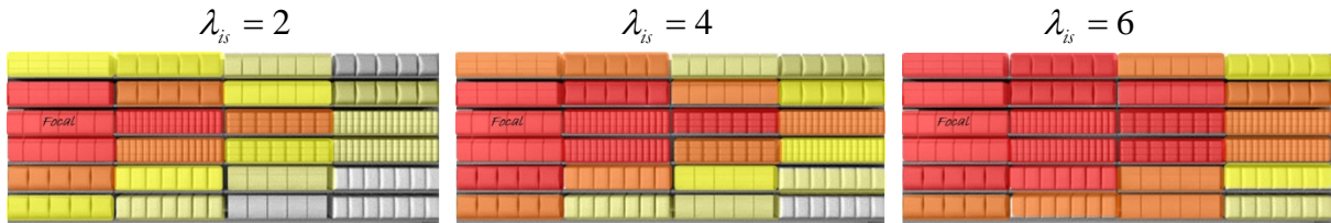
Figure 9. Consideration set with \lambda_{is} = 2, 4 and 6 .
