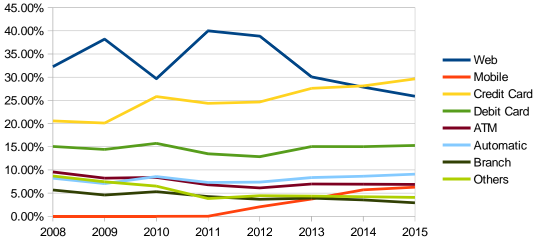
Figure 1. Channel preferences when performing current accounts and credit cards transactions.
