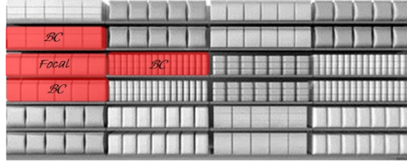
Figure 8. Focal product and its basic consideration set
