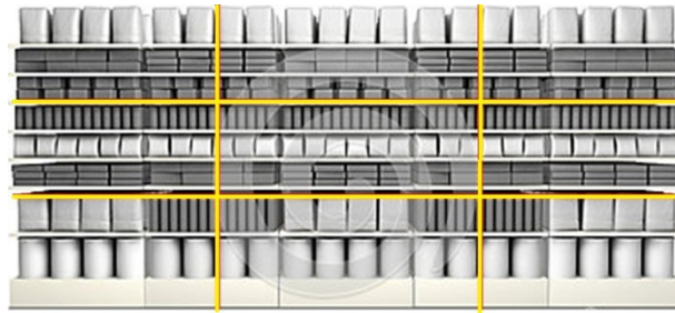
Figure 10. Location based consideration sets of the nested logit model.
