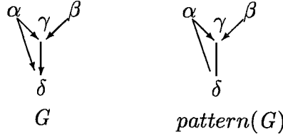
Figure 4: Graph and pattern
