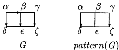
Figure 3: Chain graph and pattern
