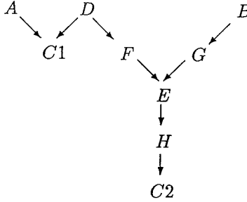
Figure 1: Schematic of singly connected graph between A and B given C = \{C1, C2\} .
