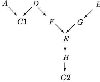
Figure 2: Graph G' .
