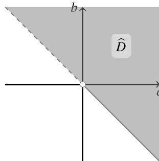
Fig. 7. A coherent maximal set of desirable gambles \widehat{D} .
