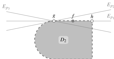
Fig. 19. g is non exposed for D_2 .
