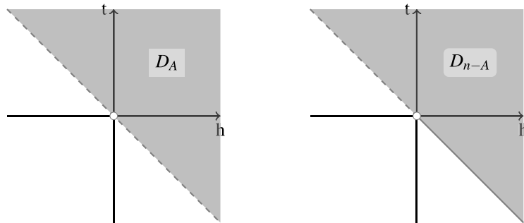
Fig. 2. An Archimedean set of desirable gambles D_A and non-Archimedean set of desirable gambles D_{n-A} .
