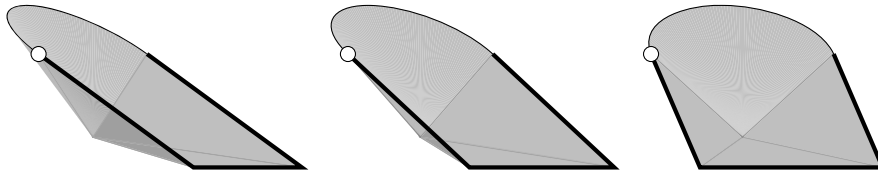
Fig. 4. An SSK-Archimedean set of desirable gambles that is not evenly convex set—viewed from three different angles.
