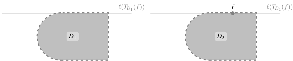
Fig. 15. The largest linear spaces \ell(T_{D_1}(f)) and \ell(T_{D_2}(f)) included in the Bouligand tangent cones of D_1 and D_2 .
