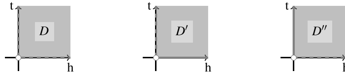
Fig. 3. An open set of desirable gambles D two sets of desirable gambles D' and D'' that are not open.
