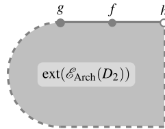
Fig. 18. The SSK-extension of \mathcal{E}_{\text{Arch}}(D_2) .
