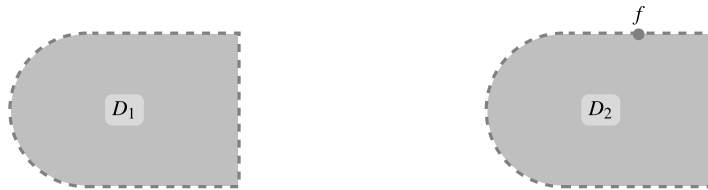
Fig. 14. The two sets of desirable gambles D_1 and D_2 .
