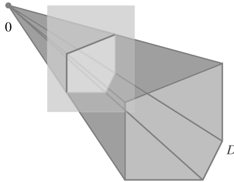
Fig. 9. A generic set of desirable gambles in a ternary space.
