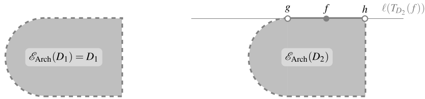
Fig. 16. The SSK-Archimedean natural extensions of D_1 and D_2 .
