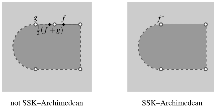
Fig. 10. A graphical representation of a non-SSK-Archimedean and an SSK-Archimedean coherent set of desirable gambles.
