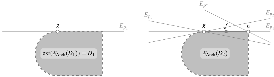
Fig. 17. g is exposed for D_1 but not for \mathcal{E}_{\text{Arch}}(D_2) , and h is exposed for \mathcal{E}_{\text{Arch}}(D_2) .
