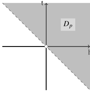
Fig. 6. A set of desirable gambles D_p corresponding to the uniform probability mass function p = (1/2, 1/2) .
