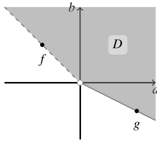
Fig. 11. The set of desirable gambles D used in Example 8.
