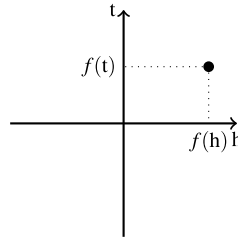
Fig. 1. A gamble f on the binary possibility space \Omega = \{h, t\} .
