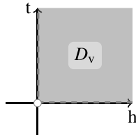
Fig. 5. The vacuous set of desirable gambles D_v .
